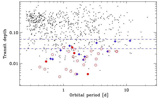
Figure 15. Transit depth versus orbital period for all systems that present transit-like features in their light curves. Black dots represent eclipsing binaries, red filled circles are our good planetary candidates, blue stars are candidates identified as eclipsing binaries and red open circles are unsettled candidates. The dashed blue lines represent our transit depth thresholds of 3 per cent and 5 per cent used as candidate selection criteria.
