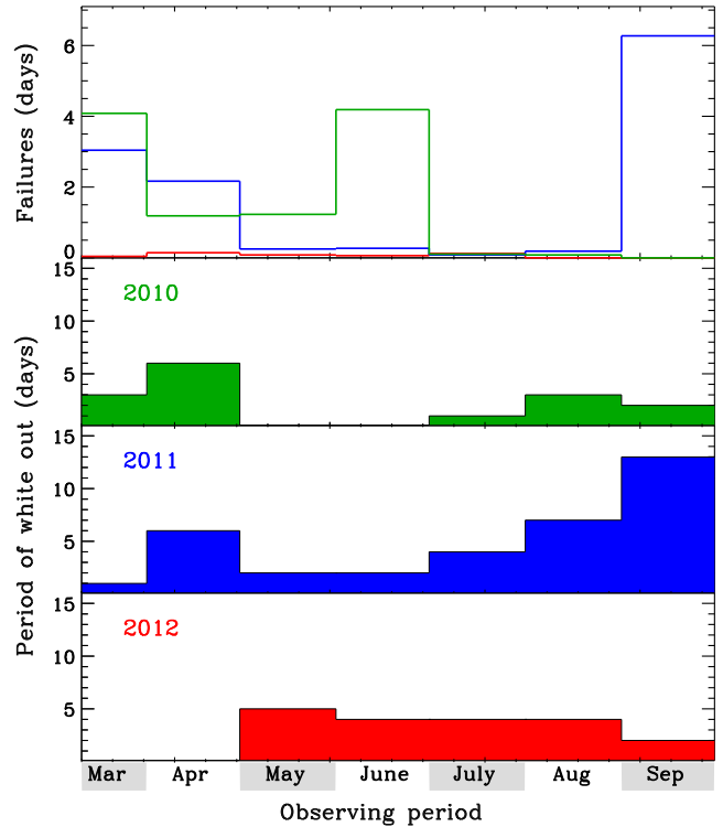
Figure 5. Monthly periods of whiteout observed at Concordia as a function of observing period in 2010 (green), 2011 (blue) and 2012 (red). The upper plot shows the period of unavailability of ASTEP-400 due to technical issues and maintenance operations of the instrument in 2010 (green), 2011 (blue) and 2012 (red). Details of the main issues are given in Table 2. Note that the 2011 September technical issue occurred during a period of whiteout.
