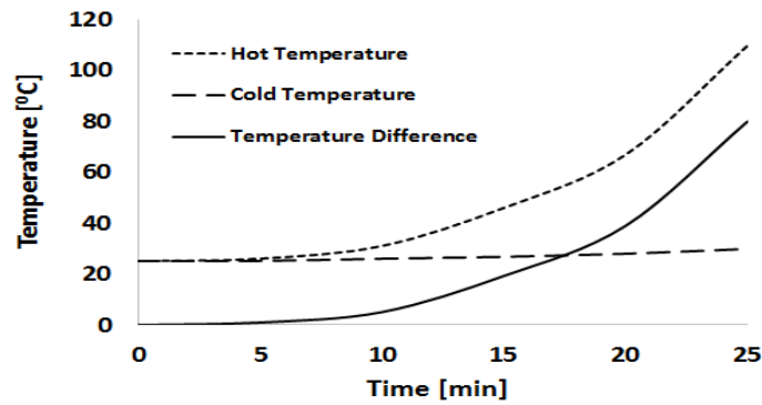
Fig. 5. Variation of temperature difference in function of time
