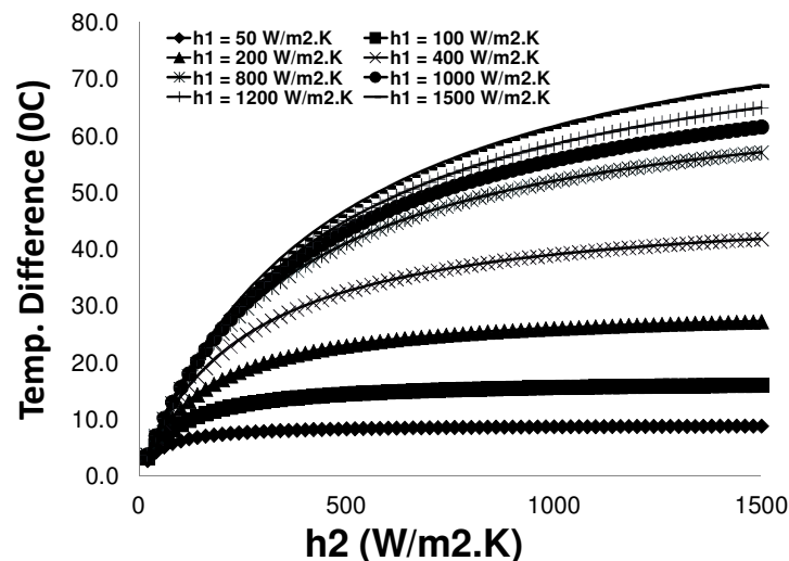
Fig. 3. Variation of the temperature gradient in function of the convective coefficients of the hot and cold fluids.
