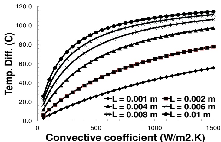
Fig. 2. Variation of the temperature gradient in function of the convective coefficient for different TEG thicknesses.
