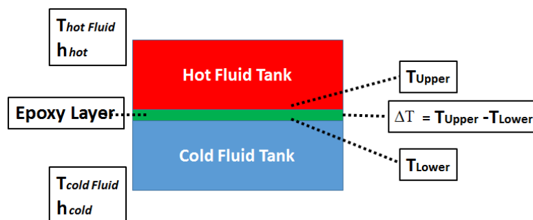
Fig. 4. Prototype simulating TEG undergoing heating and cooling by convection
