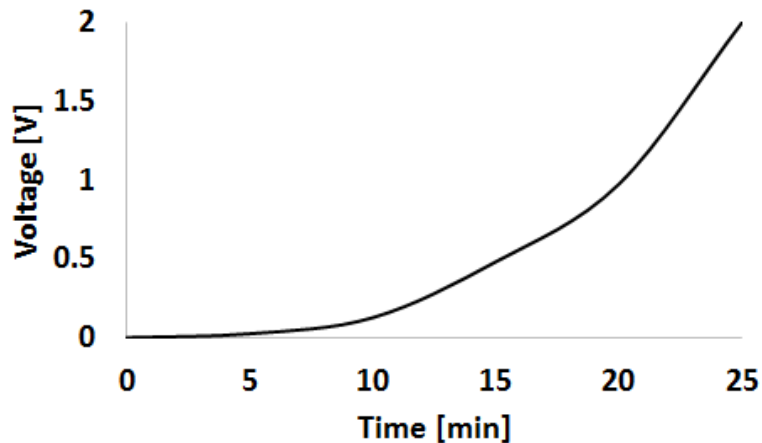
Fig. 6. Variation of voltage in function of time
