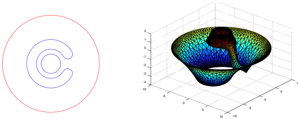
Figure 3: Example of configuration giving rise to a divergence of the method of reflections when applied to the solution of a Laplace problem with mixed (Dirichlet and Neumann) boundary conditions. Left figure: representation of the domain (with red boundary) and two objects (with blue boundaries). Right figure: numerical representation of the computed reference solution for this problem.
