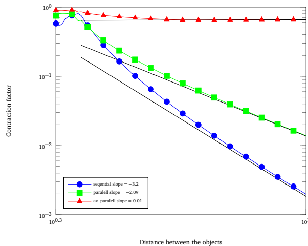
Figure 4: Plot of the value of the estimated contraction factor of the method as a function of the distance between the objects. The linear regressions are done using values associated with the five largest considered distances and are represented by black solid lines.
