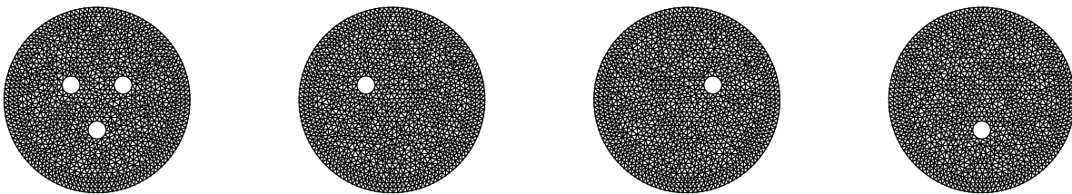
Figure 1: From left to right, finite element meshes for both the problem dealt with in Subsection 5.1 and its three associated one-object subproblems.
