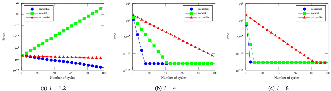
Figure 2: Relative error of the method of reflections \ell^2 -norm as a function of the number of cycles for three chosen values of the distance between the objects.
