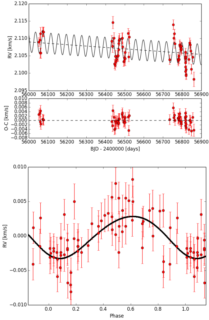
Fig. 8. Upper panel: radial velocities of HD 164595 with the best-fit orbital solution (solid line). Error bars include the photon and instrumental noise and the stellar jitter. Bottom panel: phase-folded radial velocities of HD 164595 with the best-fit orbital solution (solid line). Error bars include the photon and instrumental noise and the stellar jitter.
