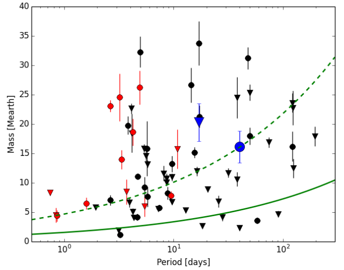
Fig. 9. Mass – orbital period of known planets with m \sin i < 40 M_{\oplus} , \Delta m \sin i / m \sin i < 0.3 . Another three planets with P > 300 days are not represented because of visibility problems. Transiting planets are shown in red, while the others are black. Triangles correspond to planets in multiplanetary systems. HD 164595b and HD 190360c are the blue circle and triangle. The green curves refer to the 3 \text{ m s}^{-1} (dashed) and 1 \text{ m s}^{-1} (solid) iso RV semi-amplitudes for a solar-type star. This diagram is based on data from the exoplanet.org database.
