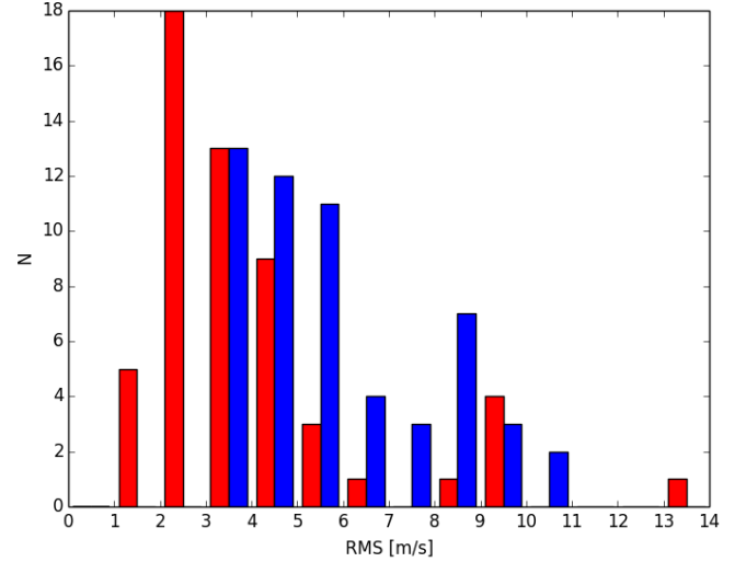
Fig. 2. Initial (blue) and final (red) distribution of the rms in the 55-star sample.
