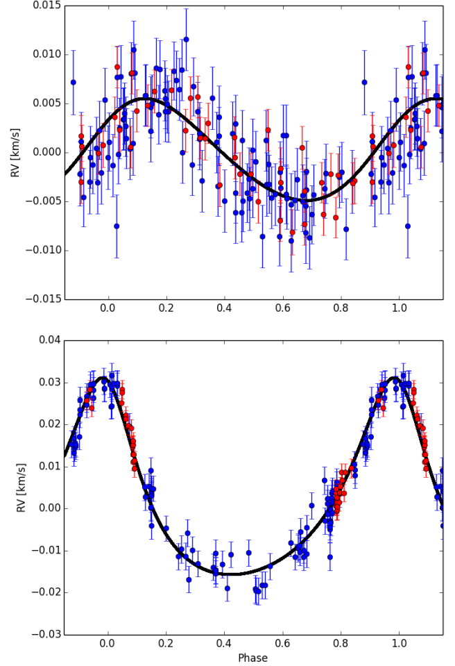
Fig. 4. Phase-folded radial velocities of HD 190360c (upper panel) and HD 190360b (bottom panel) for HIRES (blue dots) and SOPHIE (red dots) with the best-fit orbital solution (solid line). Error bars include the photon noise and jitter.
