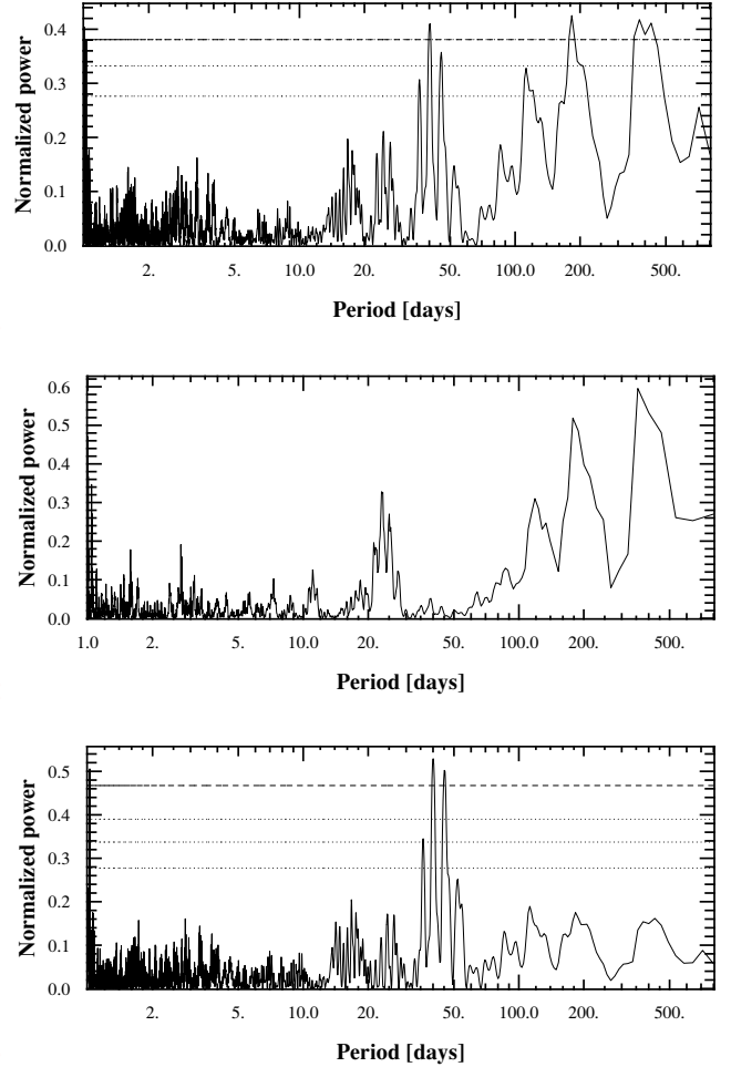
Fig. 5. Upper panel: generalized Lomb-Scargle (GLS) periodogram of HD 164595 RV before the constant master correction, with 10^{-3} FAP level (dashed line). Middle panel: GLS periodogram of the zero-point drift correction applied to HD 164595 dates of observation. Bottom panel: GLS periodogram of the corrected HD 164595 RV data, with 10^{-5} FAP level (dashed line).
