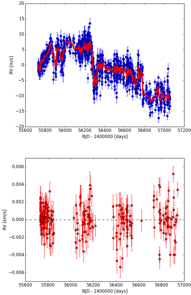
Fig. 1. Upper panel: zero-point drift correction (red line) as a function of time and the adjusted RV data set used to create it (blue dots). Bottom panel: RV time series of HD 185144 after the zero-point drift correction. This correction decreases the rms from 5.37 \text{ m s}^{-1} to 1.61 \text{ m s}^{-1} .
