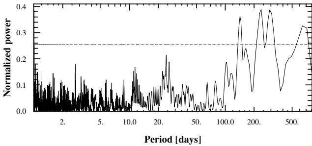
Fig. 7. HD 164595 bisector Generalized Lomb-Scargle periodogram with 0.1 FAP level (dashed line). Long-period signals above this level are caused by a trend in the last season that is marginally correlated with the radial velocities.
