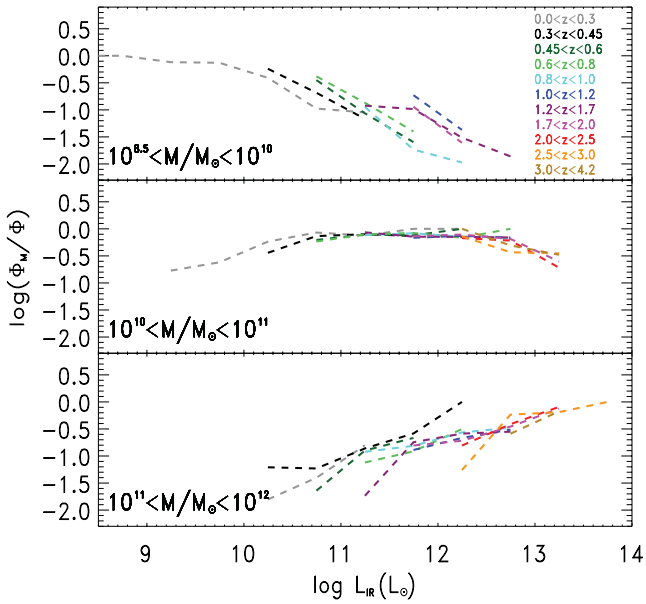
Figure 14. Ratio between the IR LF of galaxies in three different mass intervals: 8.5 < \log(M/M_{\odot}) < 10 (top); 10 < \log(M/M_{\odot}) < 11 (middle) and 11 \leq \log(M/M_{\odot}) < 12 (bottom), as shown in Fig. 13, and the total IR LF, plotted in all the different redshift intervals considered in this study, from z \sim 0 to z \sim 4 . The different colours represent the different redshifts, as explained in the plot.
