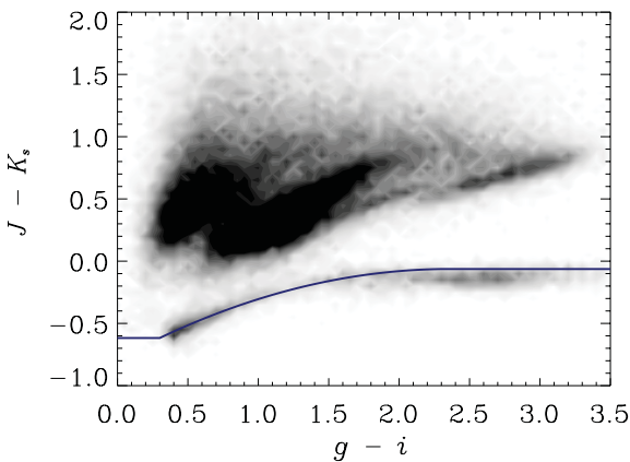
Figure 8. Colour-colour diagram showing g - i from the CFHTLS-D1 versus J - K_s for sources with K_s < 23.5 in VIDEO. The solid blue line denotes the stellar locus fit from (Baldrý et al. 2010) offset by 0.1 mag in J - K_s colour as described in the text.
