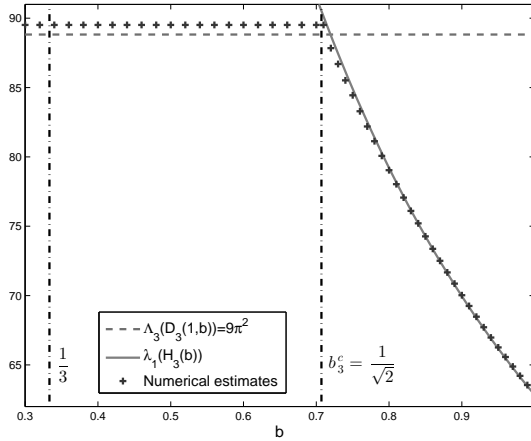
Figure 3: Upper bounds of \mathfrak{L}_3(\mathbb{T}(1, b))
