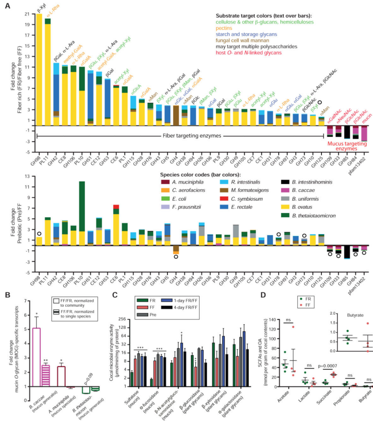
Figure 3. Diet-specific changes in carbohydrate active enzyme expression reveal a community shift from fiber to mucus degradation
