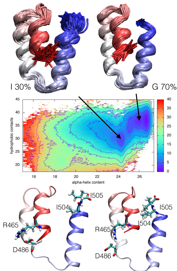
FIGURE 3. Free energy surface (in kJ/mol) of the replica-averaged meta-dynamic XD ensemble as a function of \alpha -helical content and number of hydrophobic contacts. The projection highlights a 70% populated ground state and a 30% populated intermediate state. The two states are represented as an ensemble of structures (top) as well as an average structure (bottom).
