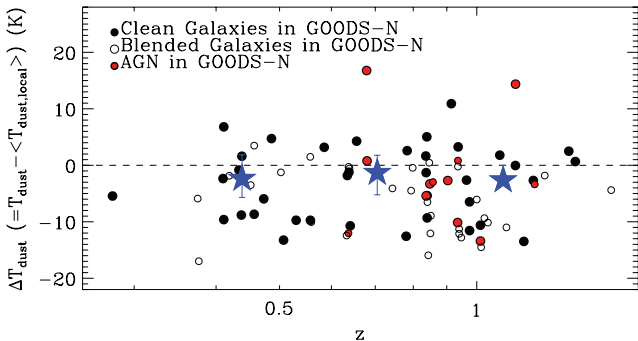
Figure 5. Deviation of T_{\text{dust}} ( \Delta T_{\text{dust}} ) for high- z LIRGs from the median trend of local LIRGs versus redshift. Filled and open symbols are ‘clean’ and ‘blended’ galaxies, respectively. Star symbol represents the median value of \Delta T_{\text{dust}} for ‘clean’ galaxies in each redshift bin.
