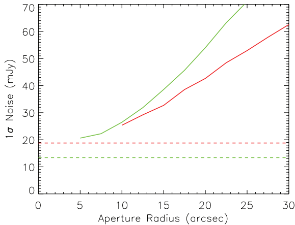
Figure 10. Continuum lines: Noise estimates for the 100- (green) and 160- \mu\text{m} (red) images as a function of aperture size. Dashed lines: The 1\sigma point-source sensitivities expected for H -ATLAS based on the HSpot observation planning tool (as shown in Eales et al. 2010).
