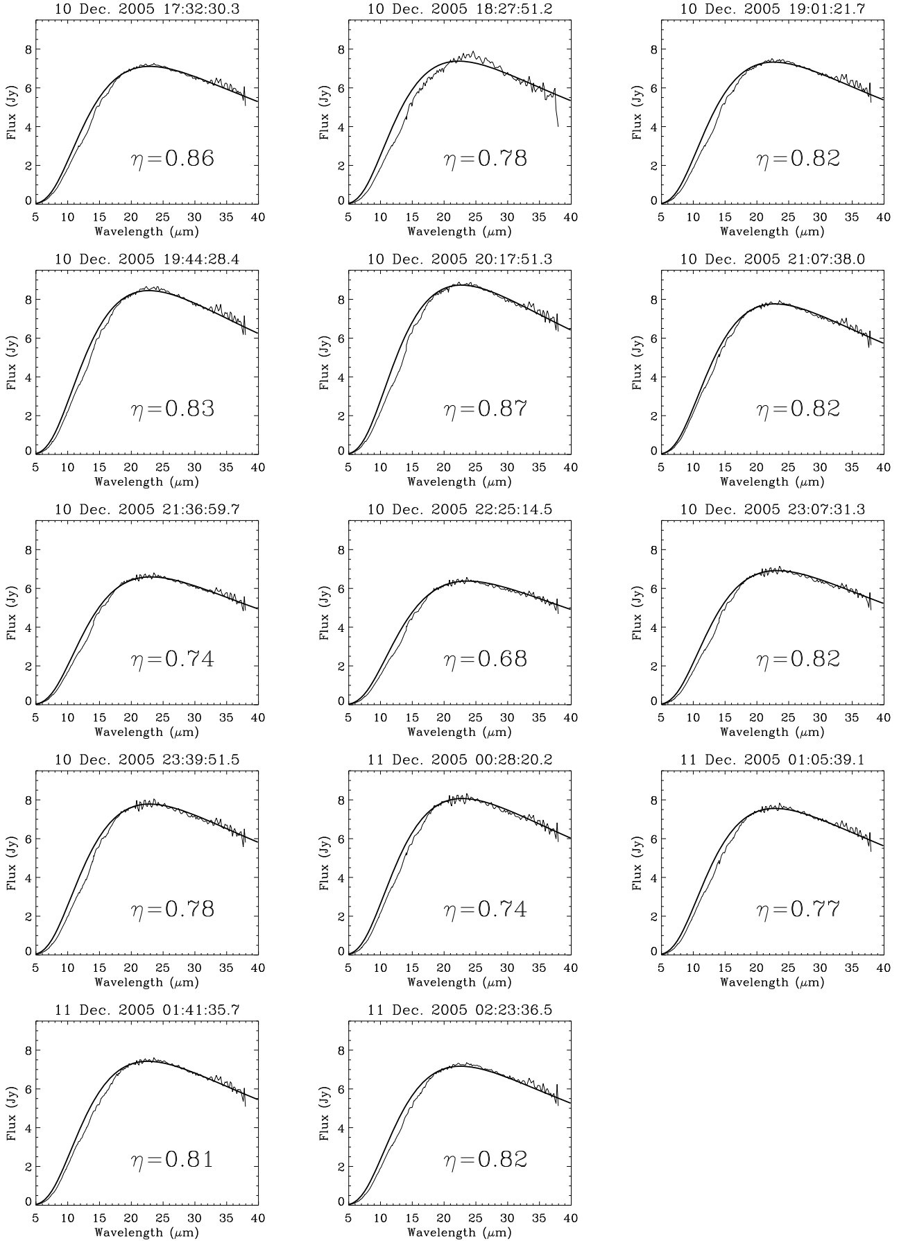
Fig. 4. The fourteen SEDs of Lutetia over the full spectral range 5–38 \mu\text{m} (thin lines). The thick solid lines correspond to the SEDs calculated with our model assuming a constant thermal inertia I = 0 and a variable value of \eta (see text for detail).
