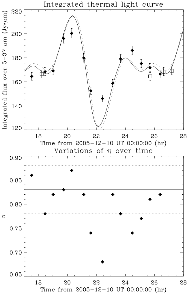
Fig. 3. Upper panel: Thermal light curves of asteroid 21 Lutetia. The symbols correspond to the SST observations (the open squares correspond to phased-folded data points). The solid line corresponds to the synthetic thermal light curve with the combination (I = 0, \eta = 0.83) , while the dotted line corresponds to the combination (I = 30 \text{ JK}^{-1} \text{ m}^{-2} \text{ s}^{-1/2}, \eta = 0.67) . Lower panel: Variations in the \eta parameter with time for a constant thermal inertia I = 0 (see Sect. 4.2 for details). The horizontal solid and dashed lines correspond to the nominal value \eta = 0.83 \pm 0.05 for I = 0 given in Table 2.
