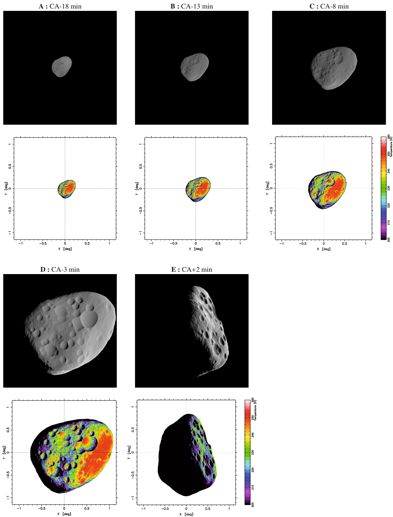
Fig. 5. Simulated visible (in black and white) and thermal (in color) images of asteroid 21 Lutetia during the forthcoming Rosetta flyby on 10 July 2010. Images were calculated at distances of 16 300 km (panel A), 11 800 km (panel B), 7600 km (panel C), 3900 km (panel D), and 3700 km (panel E) from the asteroid, corresponding to phase angles of 0°, 4°, 13°, 40°, and 110°, respectively. CA stands for Closest Approach (3055 km).
