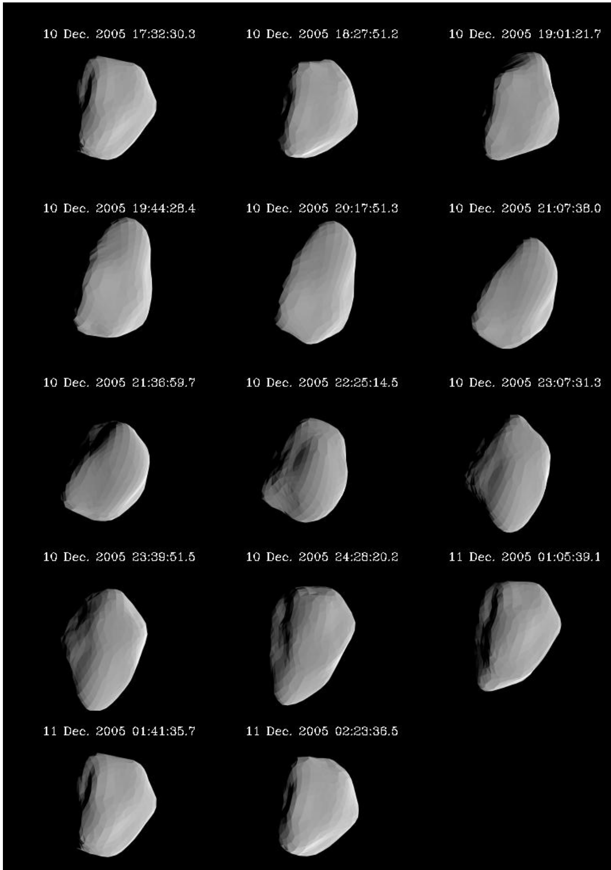
Fig. 2. Fourteen views of Lutetia as it would have appeared to the SST in the visible (i.e., reflected light) at the time of the 14 visits. The orientation is such that the aspect angle (defined as the angle between the spin vector and the asteroid-observer vector) equals 75^\circ , close to an equatorial view.
