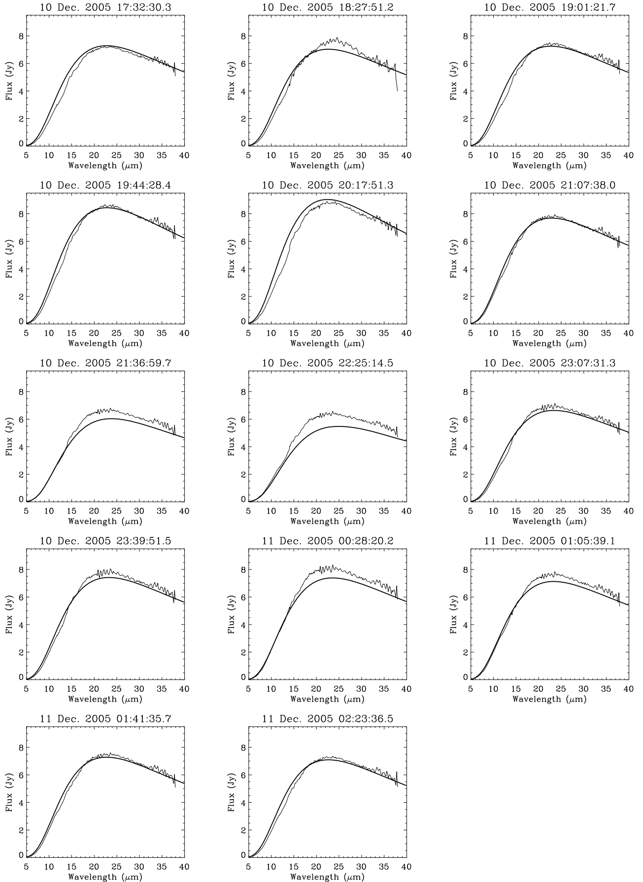
Fig. 1. The fourteen SEDs of Lutetia over the full spectral range 5–38 \mu\text{m} (thin lines). The thick solid lines correspond to the SEDs calculated with our model for the combination of thermal parameters I = 0 and \eta = 0.83 (see text for details).
