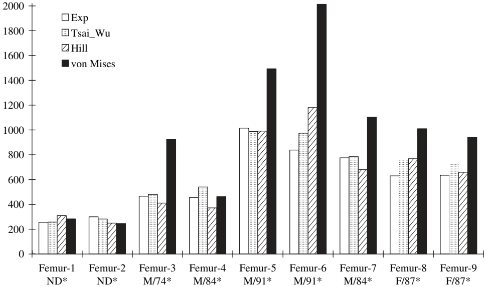
Fig. 4. Comparison of experimental measured fracture loads “ F_{exp} ” with predicted fracture loads obtained by Tsai–Wu criterion “ F_{Tsai-Wu} ,” Hill criterion “ F_{Hill} ” and Von Mises criterion “ F_{von Mises} .” *Donor’s gender and age (ND = not defined).
