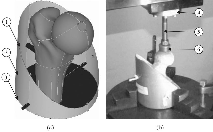
Fig. 1. (a) 3D reconstruction of the fixation device holding the proximal femur: (1) screw, (2) PVC sleeve, (3) threaded rod. (b) Device in test machine: (4) load cell, (5) metallic indenter, (6) elastomer ring. An epoxy resin (AXON F1) was used to immerged specimen in PVC sleeve.
