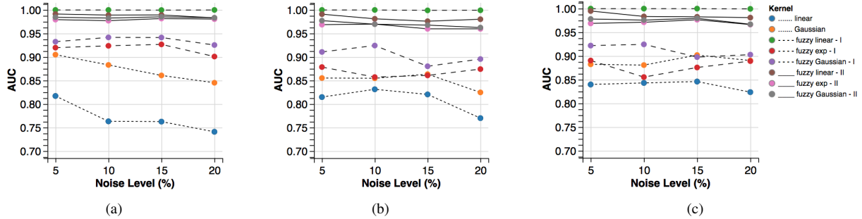
Fig. 2. Results for the PIMA attribute noise data set.
