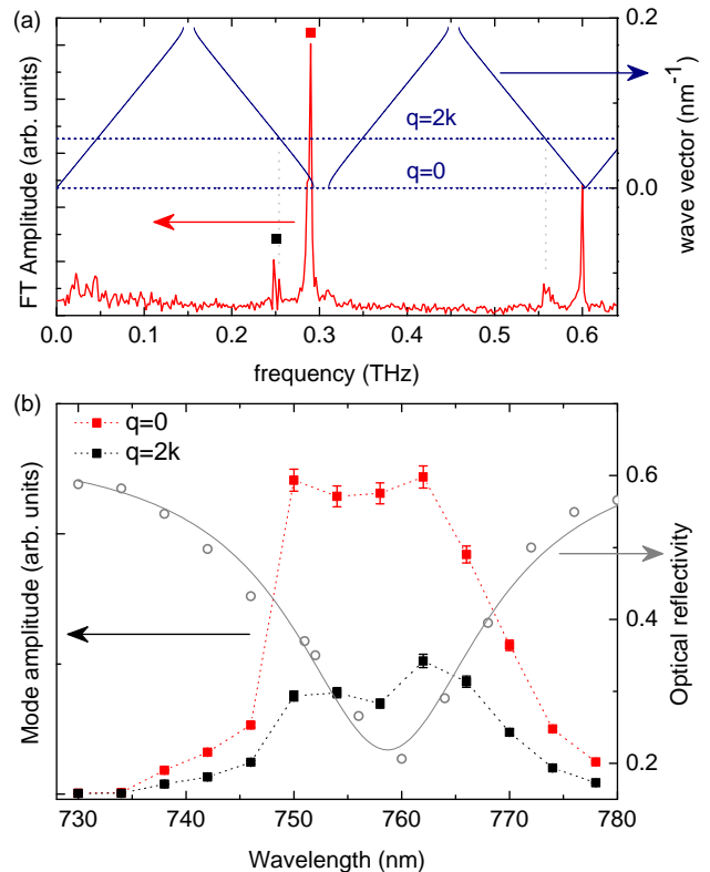
FIG. 4. (color online) In sample B, (a) FT amplitude of the change of reflectivity just after time delay zero (red line), compared to the SL dispersion curve (blue line, right scale). The laser wavelength is set to 750 nm; (b) q = 0 and q = 2k mode amplitude at 250 and 290 GHz as a function of the laser wavelength. The reflectivity curve (right scale) is reminded (experimental points (o) and calculation (solid curve)).
