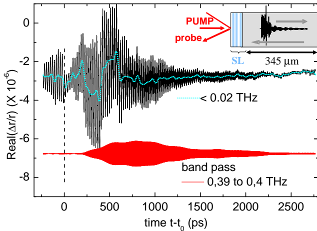
FIG. 2. (color online) In the plain SL (sample A), transient reflectivity corresponding to the first echo as a function of time delay ( t_0 \sim 144 ns is the time needed for the acoustic burst to make a round trip through the substrate, as sketched in the inset). The dotted curve is a low pass filter ( < 20 GHz), the red curve is a band pass filter about 400 GHz.
