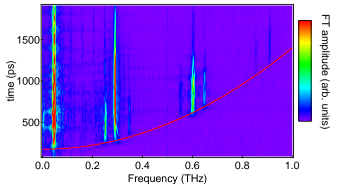
FIG. 6. (color online) In sample B, windowed Fourier Transform amplitude over 200 ps interval of the signal, as a function of the time. The red line indicates the expected arrival time.
