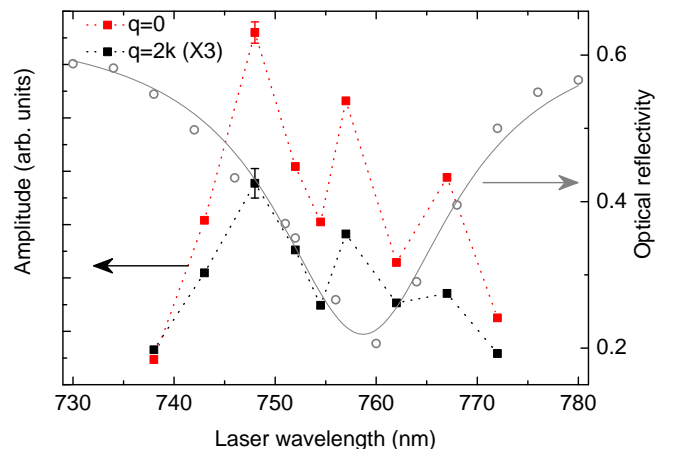
FIG. 7. (color online) In sample B, q = 0 and q = 2k mode amplitude at 253 and 290 GHz as a function of the laser wavelength (the laser intensity was set to 13 mW). The reflectivity curve (right scale) is reminded (experimental points ( \circ ) and calculation (solid curve)).
