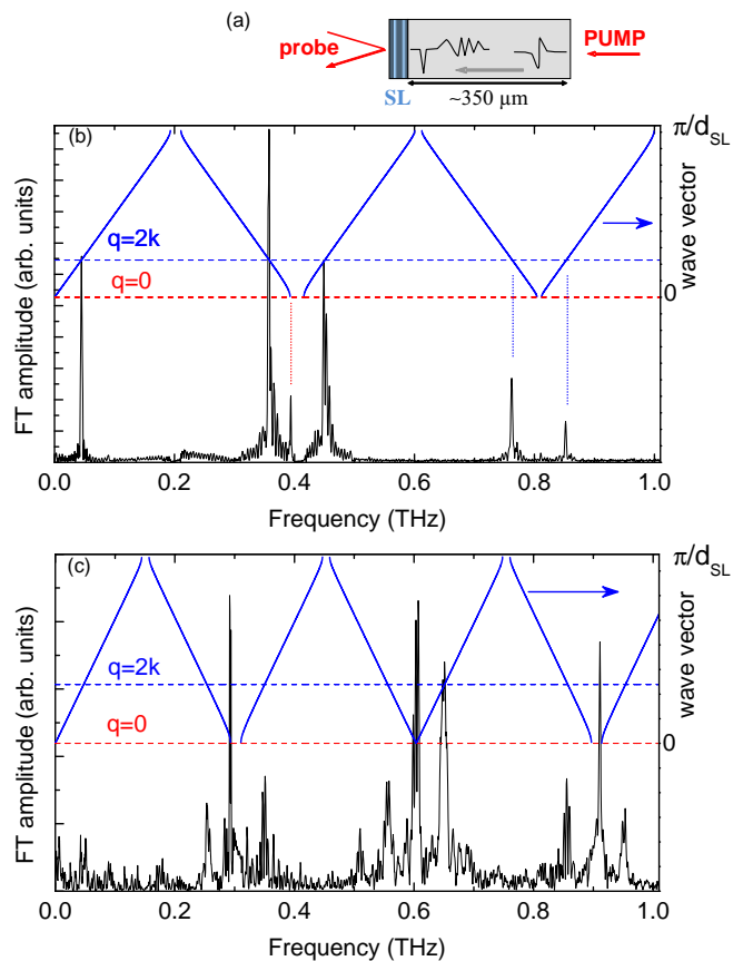
FIG. 3. (color online) FT amplitude of the change of reflectivity, compared to the SL dispersion curve (blue line, right scale), in transmission geometry (configuration (2)) as sketched in (a). (b): in sample A (776 nm) (c): in sample B (754 nm). In sample B, q = 0 modes detection is enhanced.
