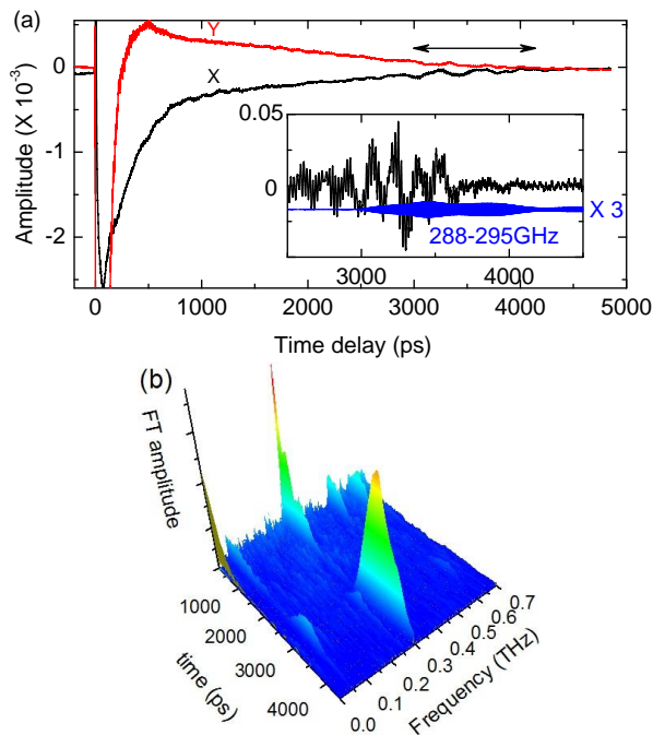
FIG. 5. (color online) In sample B, (a) Transient reflectivity \text{Re}(\Delta r/r) measured by the X and Y lock-in amplifier components (the X component is in phase with the first echo detected about a time delay of 3500 ps, after a propagation time of 152.7 ns). The laser wavelength is 758 nm (cavity mode). The arrow indicates the first echo. Inset: zoom of the echo at another laser wavelength (746 nm) with a band pass filter between 288 and 295 GHz corresponding to q = 0 mode frequency. (b) Windowed Fourier Transform amplitude over 500 ps interval of the signal, as a function of the time delay. The mode q = 0 at 293 GHz dominates the q = 2k modes (Brillouin at 48 GHz and 253 GHz), at the beginning but also in the first echo appearing after 3 ns.
