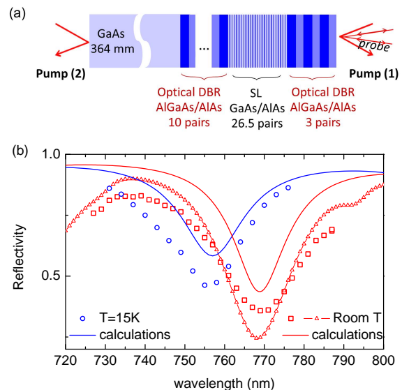
FIG. 1. (a) (color online) Scheme of the sample B, constituted by the acoustic SL inside an optical microcavity, which mirrors are the distributed Bragg reflectors (DBR). The laser beams can be focused on the structure, which is the usual experimental configuration (1), or in acoustic transmission geometry with the pump beam on the back of the substrate (2). (b) Reflectivity of the sample versus light wavelength : measurements at room temperature (red solid line with a spectrometer, red open symbols \square with the femtosecond laser), and at 15 K (shifted for clarity) (blue open symbols \circ with the femtosecond laser). The calculation done with the real structure inside the cavity is in good agreement (blue solid line).
