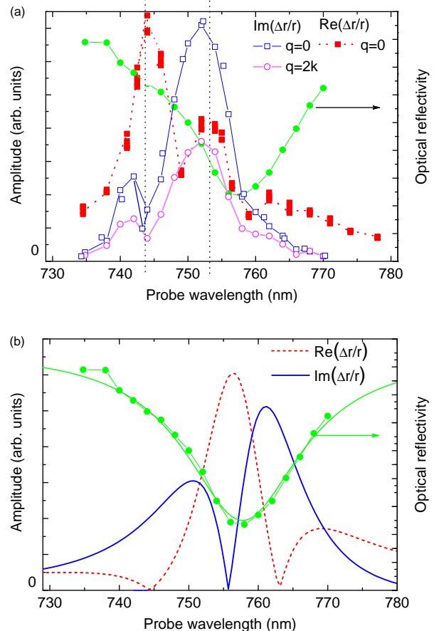
FIG. 10. (color online) In sample B, (a) FT amplitude of the q = 0 and q = 2k components of the imaginary part of the change of reflectivity due to the echo (open symbols) as a function of the probe laser wavelength. The pump beam was set at a wavelength \lambda_{\text{pump}} = 756.7 \text{ nm} . Results for the real part ( q = 0 ) are rescaled (red square) for comparison; the maxima are indicated by dotted vertical lines. Right scale: measured reflectivity. (b) Results of a simple model for the real and imaginary parts of the FT amplitude of the reflectivity change. Right scale: Reflectivity curve (calculations in solid line, measurements in symbols).
