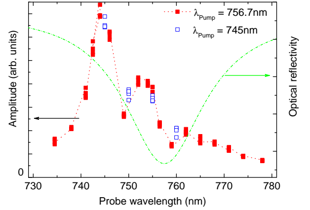
FIG. 9. (color online) In sample B, FT amplitude of the change of reflectivity due to the echo (real part) for q = 0 at 293 GHz as a function of the probe laser wavelength. The pump beam was set at a wavelength \lambda_{\text{pump}} = 756.7 nm (red square) or \lambda_{\text{pump}} = 745 nm (open blue square, \times 1.8 ). In dotted dashed line, the calculated reflectivity (right scale).
