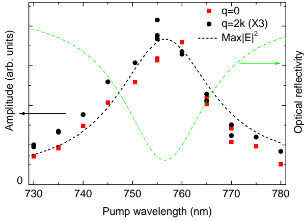
FIG. 8. (color online) In sample B, FT amplitude of the change of reflectivity due to the echo (real part) for q = 0 at 293 GHz and q = 2k lower mode ( \times 3 ), as a function of the pump laser wavelength. \lambda_{\text{probe}} = 744 nm. In dotted line, electric field square modulus calculated inside the cavity (arb. units), and in dotted dashed line, the corresponding calculated reflectivity (right scale).
