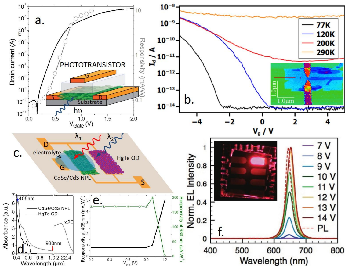
Figure 6 : a) Transfer curve (drain current vs gate bias) for a film of CdSe/CdS NPLs gated with ion gel polymer. VDS is set at 0.5V and measurements are made at room temperature in air. The inset is a scheme of the device. b) Transfer curve for a transistor made of a single PbS NPL. The inset is an AFM image of the device, reprinted with permission from reference 76 . Copyright (2012), AIP Publishing LLC. c) Scheme of a bicolor detector made of a gated film of CdSe/CdS NPLs and HgTe CQDs. d) absorption spectrum for CdSe/CdS NPLs and for HgTe CQDs. e) Responsivity at 405 nm and 980 nm as a function of gate bias for the device of part c. Adapted from reference 77 , Copyright 2014 American Chemical Society f) Electroluminescence spectra of CdSe/CdS NPLs under different biases. The inset is a picture of the device under operation. Adapted from reference 78 , copyright 2013 WILEY-VCH Verlag GmbH.
