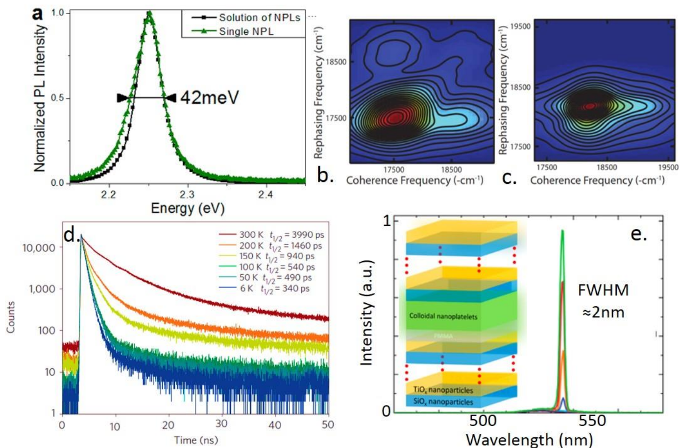
Figure 5 : (a) PL spectrum of a single CdSe NPL and of an assembly of them at room temperature. Reprinted with permission from ref 61 . Copyright 2012 American Chemical Society. 2D electronic spectrum of colloidal spherical QDs (b) and NPLs (c). Reprinted with permission from ref 62 . Copyright 2013, AIP Publishing LLC. (d) Time resolved PL spectra of CdSe NPLs at different temperature. Reprinted by permission from Macmillan Publishers Ltd. Nature Material in ref
