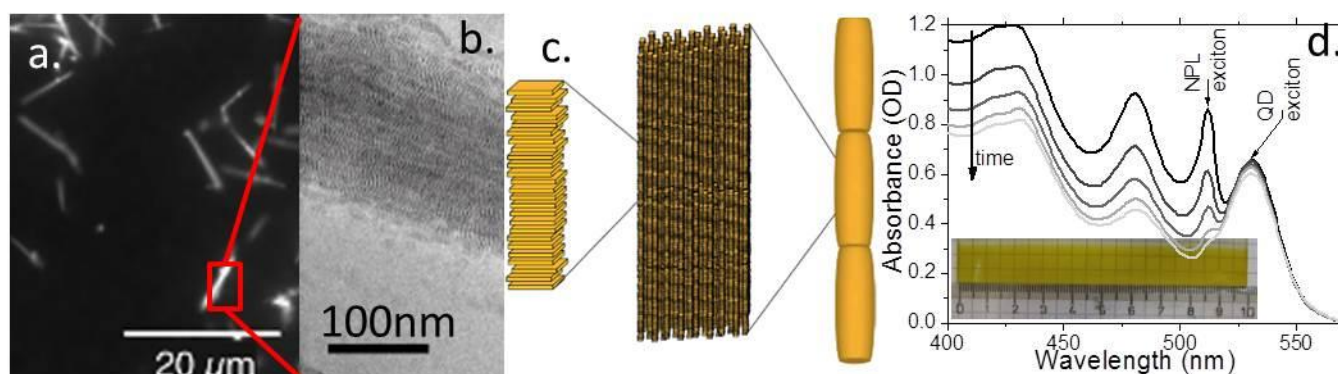
Figure 4. (a) Optical microscopy and (b) TEM images of CdSe nanoplatelets superlattices. (c) Scheme representing the hierarchical structure of the superlattices. Adapted with permission from ref 59 . Copyright (2014) American Chemical Society. (d) Absorption spectra of a mixture made of QDs and NPLs at different time during the electrophoresis of the mixture. The inset is a film of NPLs deposited using electrophoresis. The scale is in cm.
