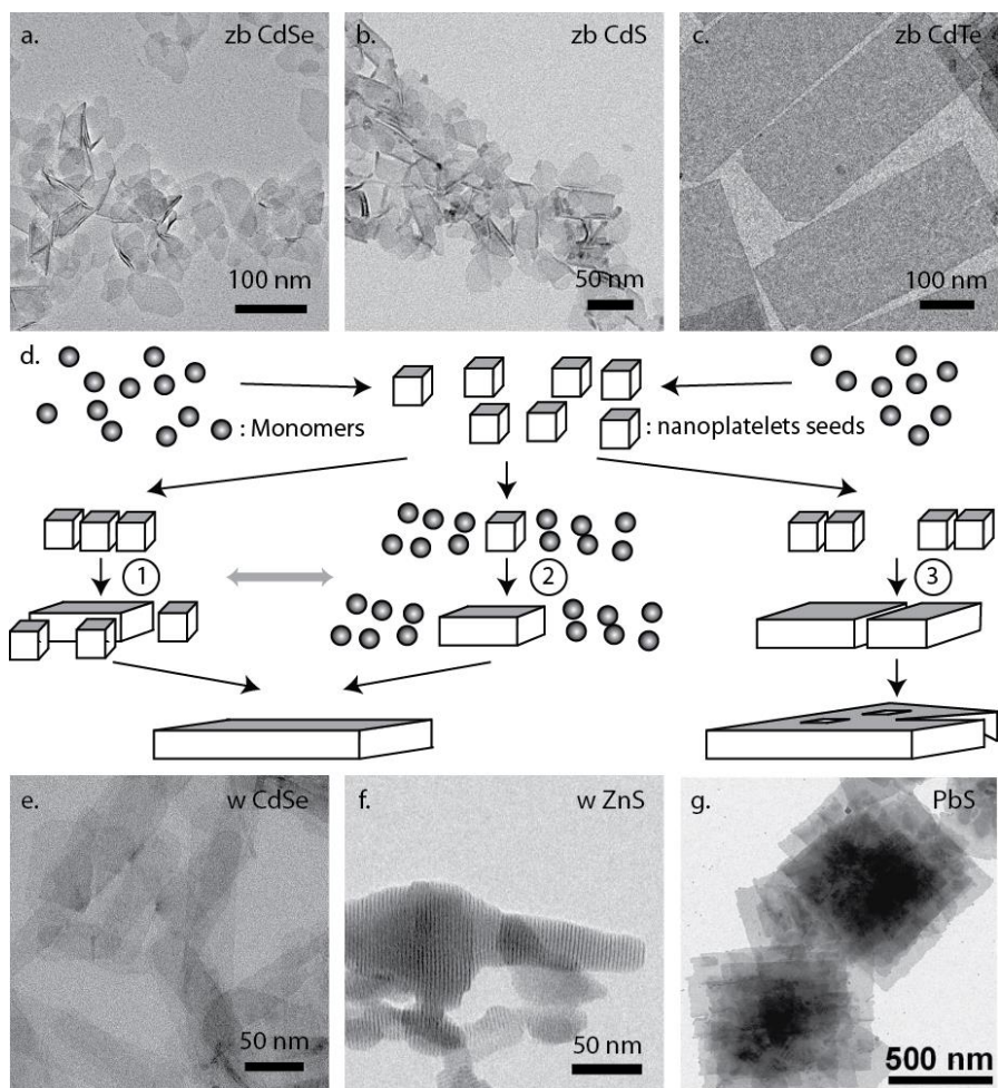
Figure 1: TEM images of zinc blende CdSe (a) CdS (b), CdTe (c) wurtzite CdSe (e) and ZnS (f), and rock salts PbS (g) NPLs, from ref 23 . Reprinted with permission from AAAS. d). Scheme of the different paths for the growth of nanoplatolets. Adapted with permission from reference 24 . Copyright (2011) American Chemical Society
