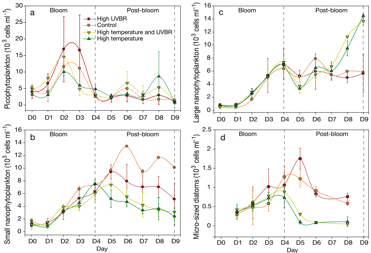
Fig. 5. Average ( \pm SD) (a) picophytoplankton abundance (cells \text{ml}^{-1} ), (b) small (2–10 \mu\text{m} ) nanophytoplankton abundance (cells \text{ml}^{-1} ), (c) large (10–20 \mu\text{m} ) nanophytoplankton abundance (cells \text{ml}^{-1} ), and (d) micro-sized (>20 \mu\text{m} ) diatom abundance (cells \text{ml}^{-1} ) in the experimental mesocosms (see Fig. 2 for descriptions of the 4 treatment groups)
