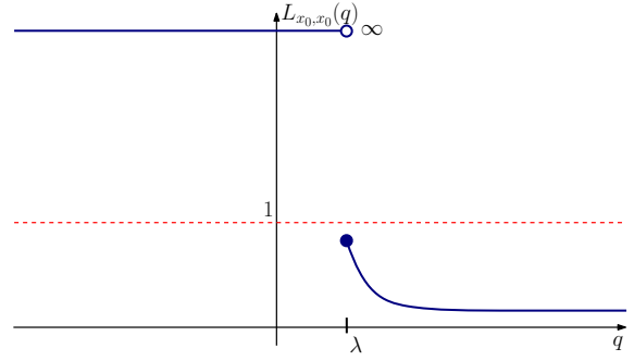
(b) A case in which condition (17) does not hold. The Malthus exponent \lambda can be defined, but we have L_{x_0, x_0}(\lambda) < 1 .
