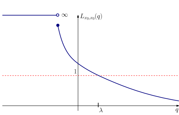
(a) A case in which condition (17) holds, as does the even stronger condition (18).
