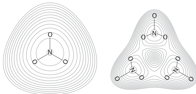
FIG. 2. Pictorial views of the \text{NO}_3^- anion (left panel) and distorted \text{NO}_3 radical (right panel) geometries superimposed on potential contour plots ( \text{NO}_3^- ground state on the left and lower adiabatic sheet of the {}^2E'' state on the right).
