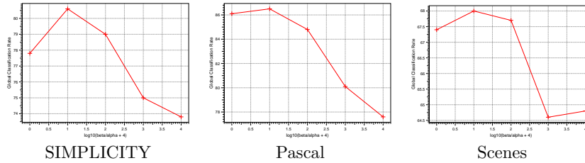
Fig. 9. evolution of the global classification rate with \frac{\beta}{\alpha}
