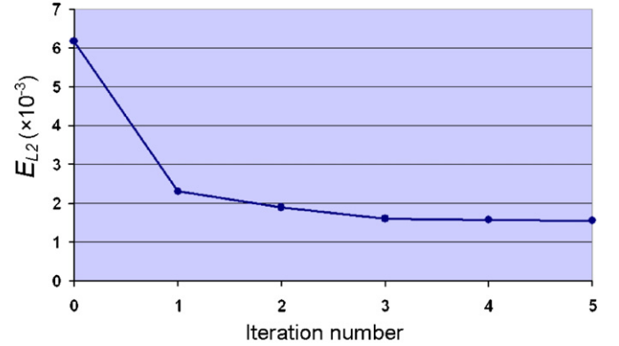
Fig. 11. Evolution of the root mean square error E_{L2} , along with the number of optimization iterations, for the RockerArm approximating surface.
