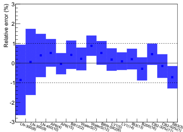
Fig. 5: RED accuracy and precision results for each insert of the Gammex 467 phantom (78 kV, 94 kV, 0.1 mm Sn) for the 20 mGy acquisition.
