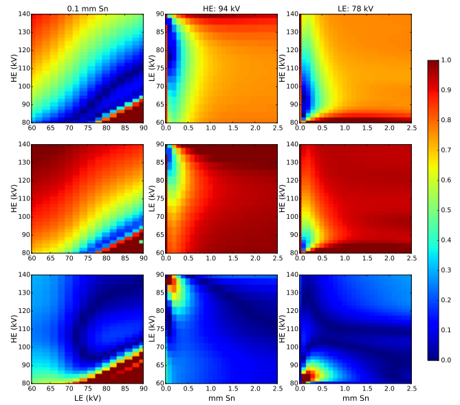
Fig. 6: From top to bottom, RED accuracy results as a function of the LE, HE and tin filtration for the insert: LN450, AP6 and CB2-50. From left to right: LE-HE plot at 0.1 mm Sn, LE-mm Sn plot at HE: 94 kV, HE-mm Sn plot at LE: 78 kV. The colorbar indicates the percentage error for the accuracy. Data corresponding to the ideal situation, without noise.
