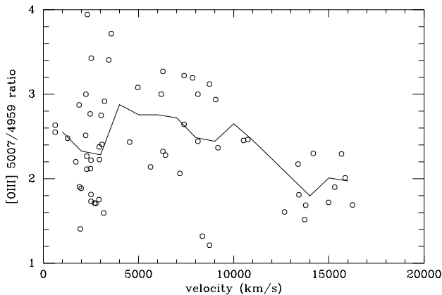
Fig. 6. Dependence [OIII] \lambda 5007/\lambda 4959 ratio on the velocities. The line relies the mean [OIII] ratio value every 1000 \text{km s}^{-1}
