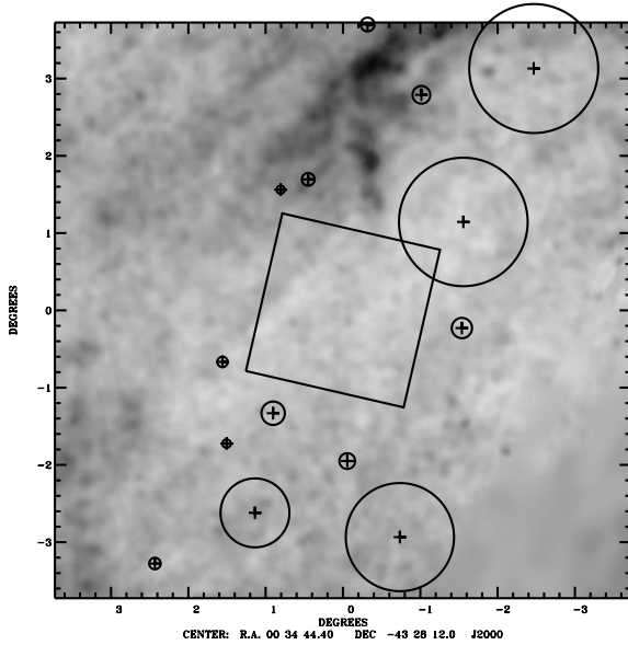
Figure 11. The location of the S1 ELAIS survey field overlaid on the COBE normalized IRAS maps of Schlegel et al. (1998). IRAS sources with 12- \mu m fluxes brighter than 0.6 Jy are overlaid with radius proportional to flux for S_{60} < 10 Jy. The minimum 100- \mu m intensity shown is 0 MJy sr ^{-1} (white) and the maximum is 1.5 MJy sr ^{-1} (black).
