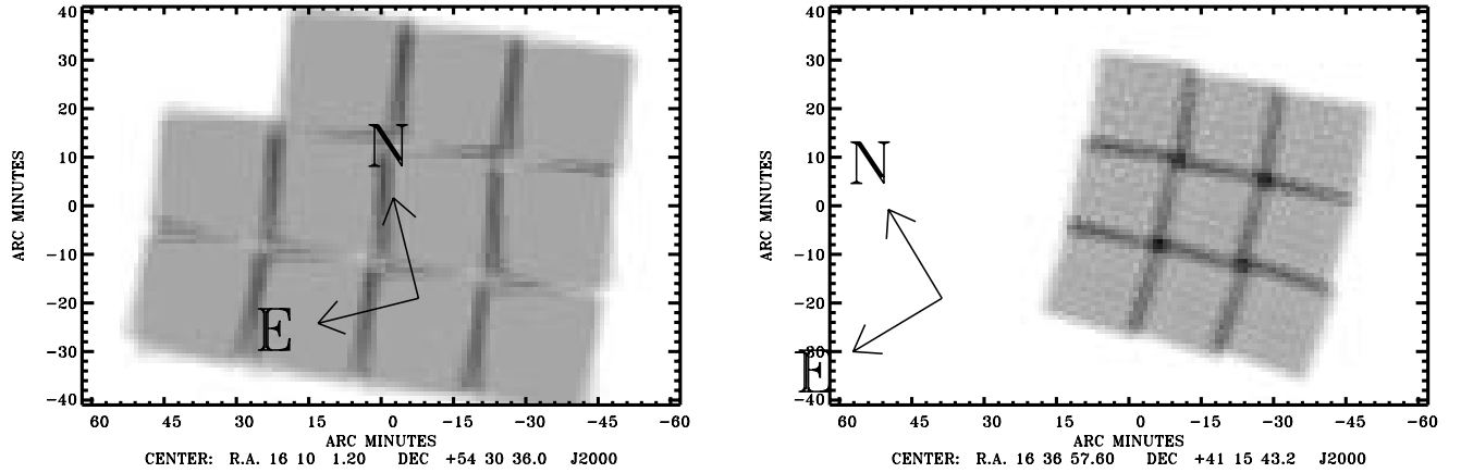
Figure 15. Survey coverage at 175 \mu\text{m} . NB Only the coverage in N2 is part of the ELAIS project, the coverage in N1 (left) comes from the FIRBACK team (PI J-L. Puget, see Dole et al. 1999). White areas have not been covered at all; darker regions indicate longer total integration, either because of repeated observations or overlap, black indicates 350 s. The coverage maps have been smoothed to 1 arcmin resolution. The true peaks in the coverage are around 260 and 350 s respectively.
