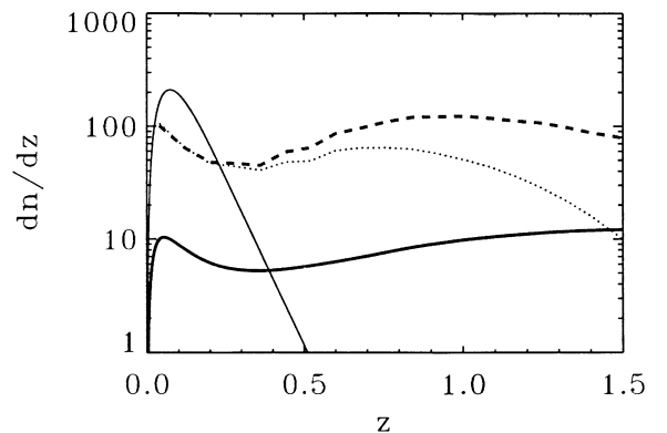
Figure 3. Expected populations and redshift distribution for the 175- \mu\text{m} survey, assuming a depth of 75 mJy over 1 \text{deg}^2 . The redshift distribution is plotted as dn/dz in dimensionless units. Cirrus (solid line) and starburst (thick solid line) components are from a model similar to Oliver et al. (1992) and Pearson & Rowan-Robinson (1996), model E (dashed line) and model A (dotted line) are from Guiderdoni et al. (1998).
