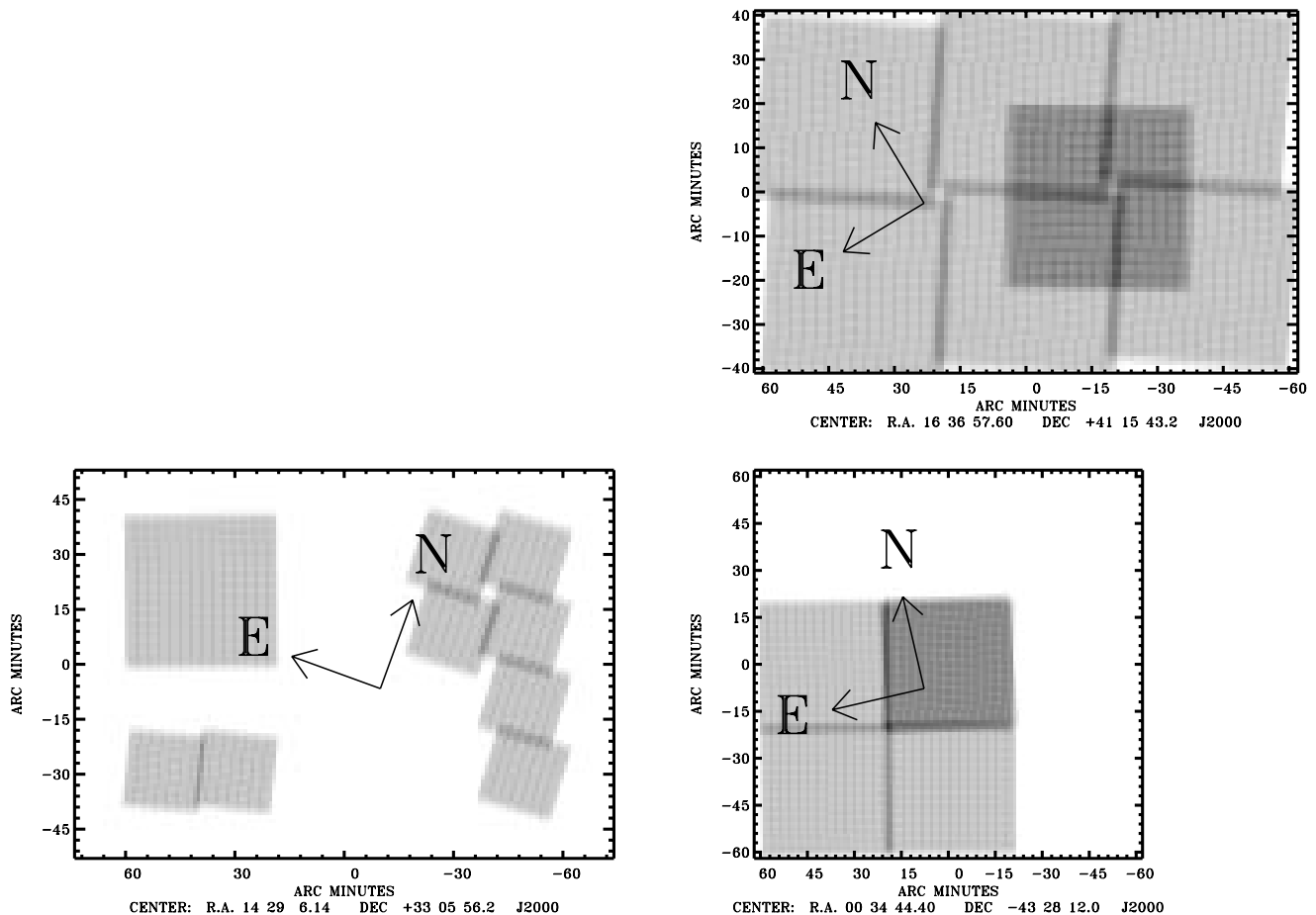
Figure 12. Survey coverage at 6.7 \mu\text{m} . White areas have not been covered at all; darker regions indicate longer total integration, either because of repeated observations or overlap, black indicates 200 s. The coverage maps have been smoothed to 1 arcmin resolution. Reading from top left to bottom right the fields are: N2, N3, S1. The true peaks in the coverage are around 150, 100 and 175 s respectively.
