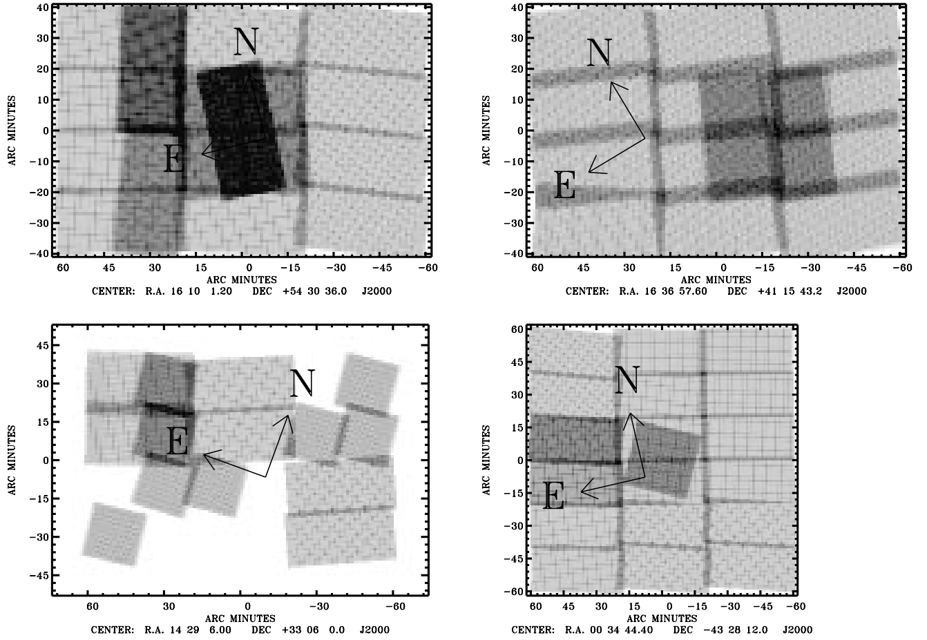
Figure 14. Survey coverage at 90 \mu\text{m} . White areas have not been covered at all; darker regions indicate longer total integration, either because of repeated observations or overlap, black indicates 100 s. The coverage maps have been smoothed to 1 arcmin resolution. Reading from top left to bottom right the fields are: N1, N2, N3, S1. The true peaks in the coverage are around 160, 120, 120 and 120 s respectively.
