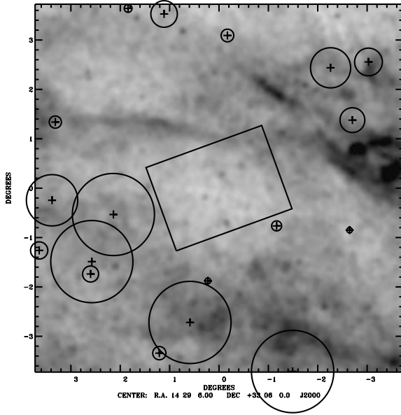
Figure 10. The location of the N3 ELAIS survey field overlaid on the COBE normalized IRAS maps of Schlegel et al. (1998). IRAS sources with 12- \mu m fluxes brighter than 0.6 Jy are overlaid with radius proportional to flux for S_{60} < 10 Jy. The minimum 100- \mu m intensity shown is 0 MJy sr ^{-1} (white) and the maximum is 1.5 MJy sr ^{-1} (black).
