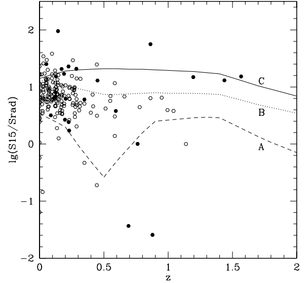
Figure 19. 15- \mu\text{m}/20\text{-cm} colour versus z for ELAIS Catalogue sources, with loci for cirrus (C, solid line), starburst (B, dotted line) and Arp220 (A, broken line) SEDs. Filled circles: AGN; open circles: galaxies.
