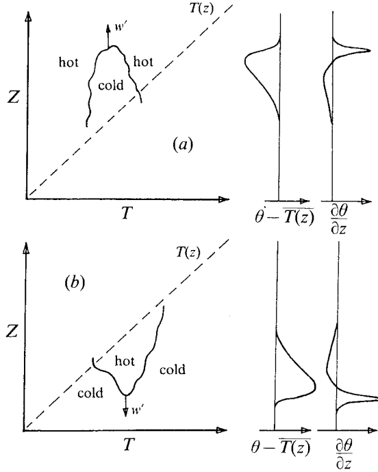
FIG. 1. Phenomenological model of fluid lumps explaining ramp-cliff events in the scalar signal and connected jumps in the instantaneous scalar derivative under influence of a mean scalar gradient [taken from Thoroddsen and Van Atta (1992) (Ref. 25) in which the scalar is temperature].
