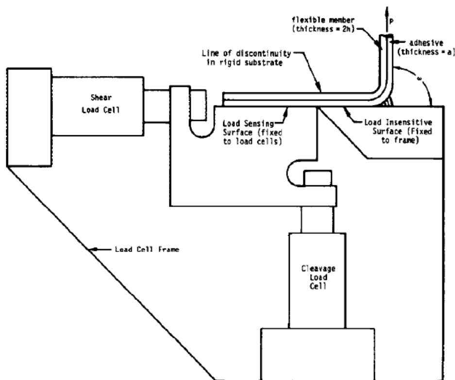
37 38 Figure 15: Schematic of the peeling device from Kaelble (1974) where the left half of the substrate beam is connected with 39 two shear and traction load cells.
