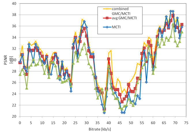
Fig. 3. Side Information PSNR for “Foreman”.
