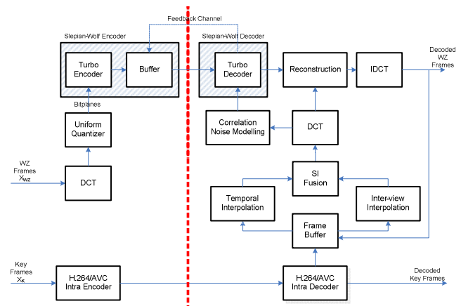
Fig. 1. Proposed multi-view DVC architecture.
