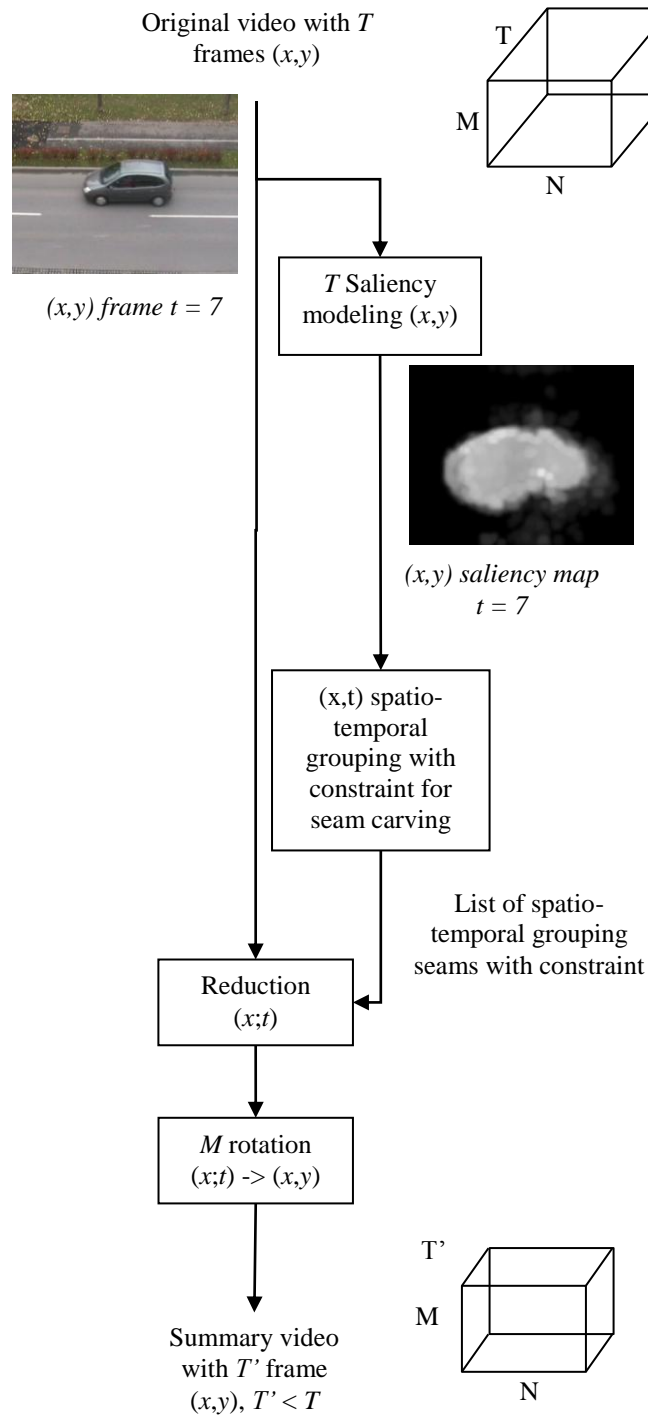
Fig. 1 Proposed approach of video summary with spatio-temporal grouping constraint for seam carving.
