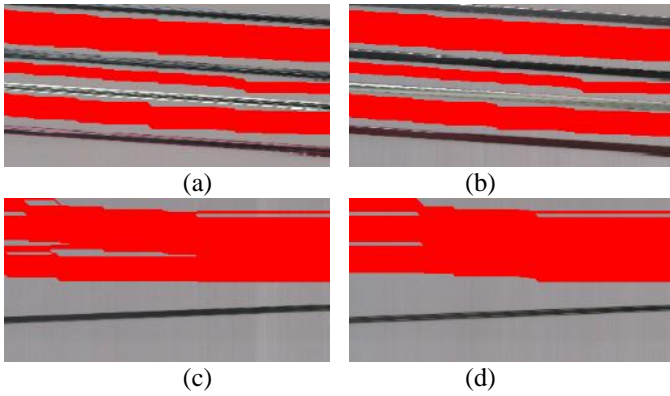
Fig. 4 Visualization of the (x,t) plane for video-A (a) y=139 , (b) y=154 , (c) y=244 , (d) y=253 ; the suppressible seams are in red, the road is in grey, and the different vehicle trajectories are in black or white.
