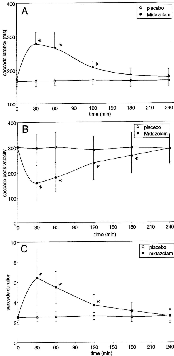
Fig. 4. Time-course of saccade characteristics after injection. Conventions are the same as in Fig. 1. A: average saccadic latency vs time after injection. B: average slope of peak velocity and amplitude vs time after injection. C: average slope of saccade duration and amplitude vs time after injection.
