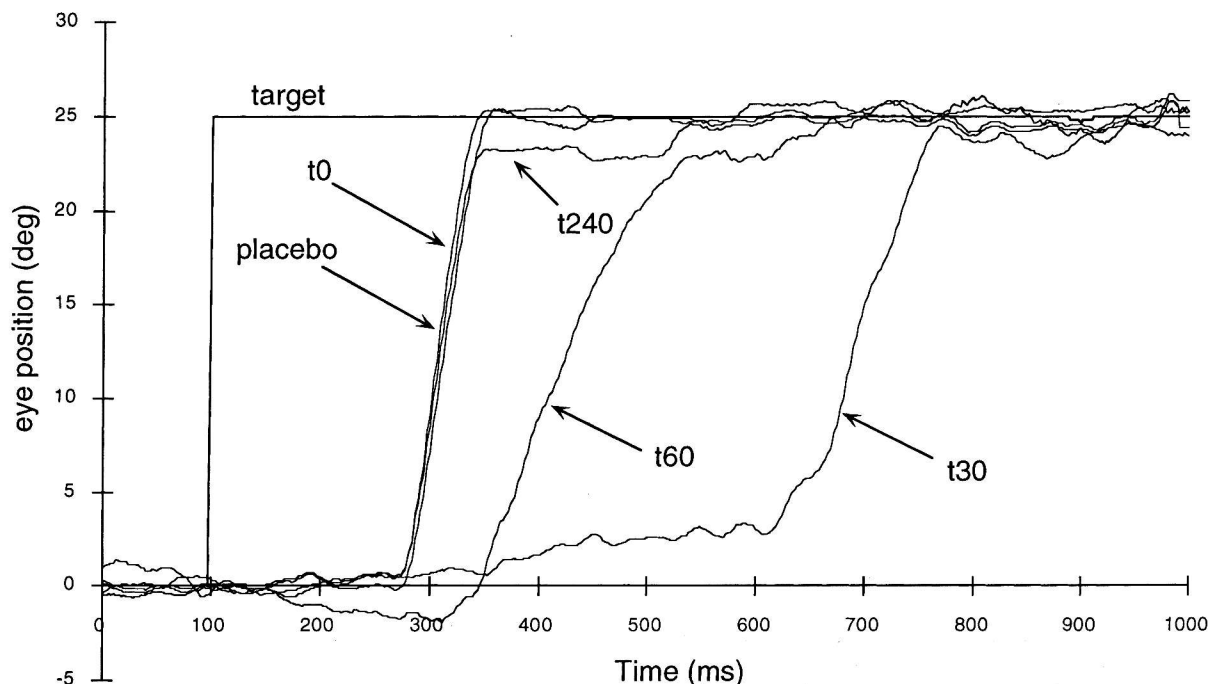
Fig. 2. Typical saccades recorded during periods pre- and post-drug administration for a 25^\circ target jump to the right. Five saccades are represented: 30 min after administration of the placebo, prior to midazolam administration (t0), then 30 min (t30), 1 hour (t60) and 4 hours (t240) after midazolam administration. The thick line represents the target position signal.
