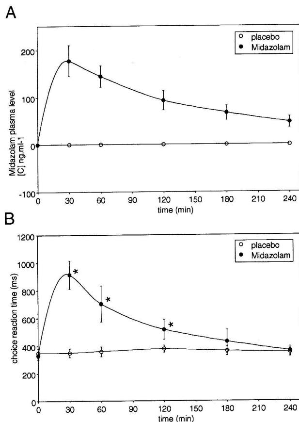
Fig. 1A. Midazolam plasma concentration as a function of time after injection. 1B: Choice-reaction-time as a function of time after injection. Data are the mean value and standard deviation over all eight subjects. Open circles (○) correspond to placebo tests, black filled circles (●) correspond to midazolam tests. (*) P < 0.05 in comparison to baseline (t 0 ) by repeated measures ANOVA and paired t -test with Bonferroni's correction.
