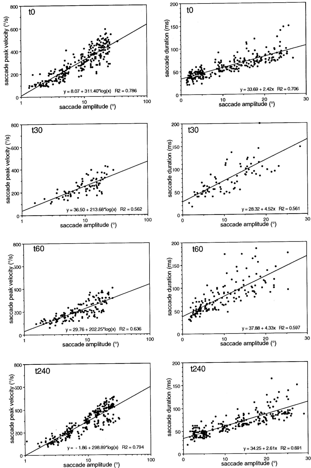
Fig. 3. Relationships between saccade amplitude and saccade peak velocity (left hand graphs) and saccade duration (right hand graphs), before (t0), 30 min (t30), 1 hour (t60) and 4 hours (t240) after administration of midazolam.
