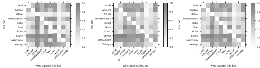
Fig. 5. Win percentages of CIG 2012 competition, from left to right: 3-player maps only, 6-player maps only, all maps. Read from line to column, bot in row wins given fraction of games against bot in column. For some bots, we find interesting differences, e.g. Xelnaga gets worse on 6-player maps, UAlbertaBot gets better. Only Xelnaga can reliably beat Skynet, but only on 3-player maps
