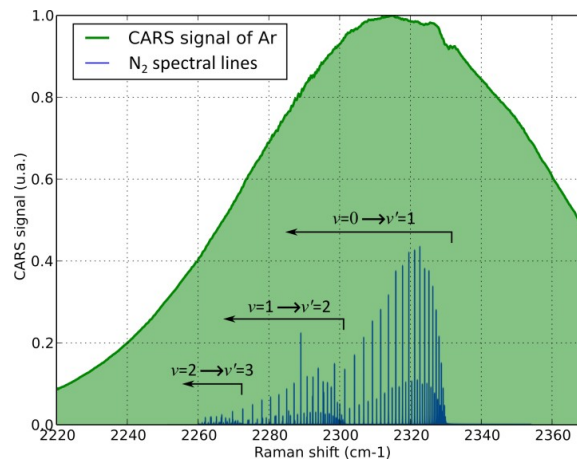
Figure . Nonresonant CARS signal of Ar (green filled curve), illustrating the bandwidth effectively excited by pump and Stokes pulses, compared to the theoretical CARS spectrum of \text{N}_2 in a flame (blue lines).
