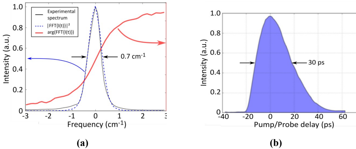
Figure - (a) Spectral and (b) temporal characterization of the generated probe pulse through the filtering stage. (a) The experimental spectrum (thin solid line) is compared to the intensity (dotted line) and phase (thick solid line) of the Fourier transform of the temporal profile.
