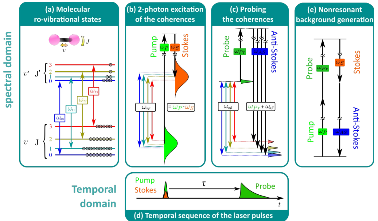
Figure 1. Sketch of the light-matter interaction in hybrid fs/ps-CARS. (a) Energy level diagram of the N 2 rotational ( J ) and vibrational ( v ) structure, and Q-branch associated Raman
