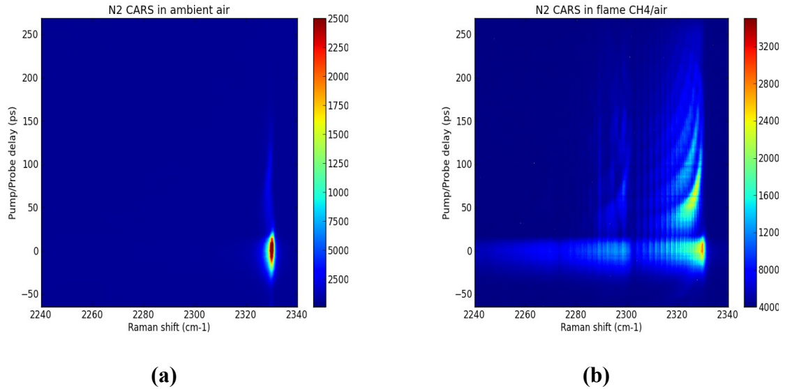
Figure – Experimental investigation of the N 2 CARS spectrum (horizontal axis) evolution versus the pump/probe delay (vertical axis) (a) in ambient air, and (b) in a CH 4 /air flame.
