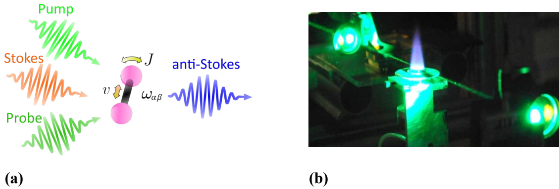
Figure . (a) Sketch of the CARS process: generation of an anti-Stokes signal by a N_2 molecule, with rotational and vibrational degree of freedom designated by their respective quantum number J and v , excited by three laser pulses, pump, Stokes and probe. (b) Illustration of CARS diagnostics in a CH_4 /air flame.
