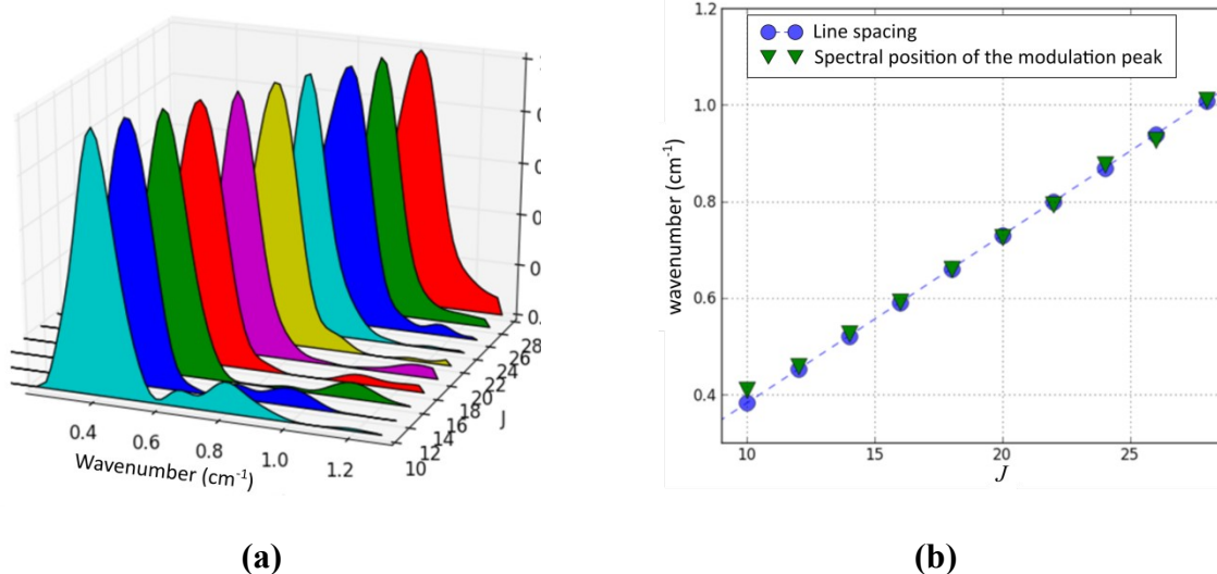
Figure – Spectral analysis of the rotational line modulation on the first vibrational band. (a) Spectral modulation peak obtained by Fourier transform of the line CARS intensity temporal evolution as a function of the rotational quantum number J, and (b) comparison of the peak position (triangle) obtained experimentally with the local spectral interval between two successive Raman lines (circle), calculated using spectroscopic constants, as a function of J.
