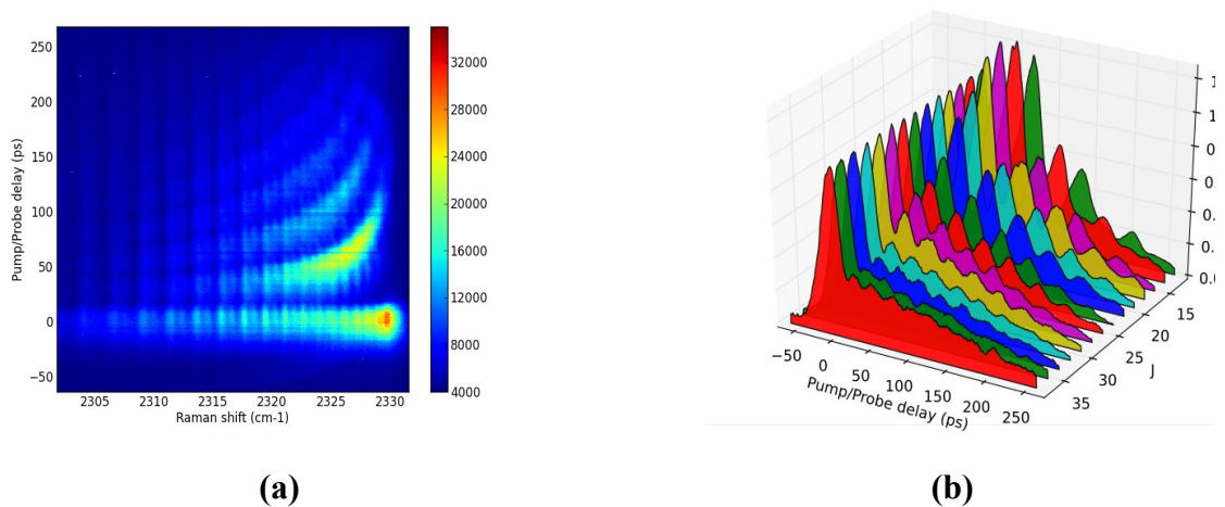
Figure - (a) Evolution of the N 2 CARS spectrum (horizontal axis) centered on the fundamental vibrational band versus the pump/probe delay (vertical axis). (b) Evolution of the
