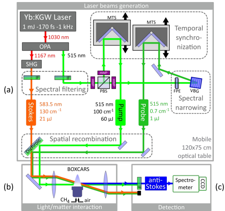
Figure . Experimental setup: (a) laser beam generation, (b) light-matter interaction in the \text{CH}_4/\text{air} premixed flame with planar BOXCARS geometry, (c) anti-Stokes detection. OPA: Optical Parametric Amplifier, SHG: second harmonic generation, IF: interferential filter, PBS: polarizing beam splitter, HWP: half-wave plate, FPE: Fabry-Perot etalon, VBG: volume Bragg grating, MTS: motorized translation stage.
