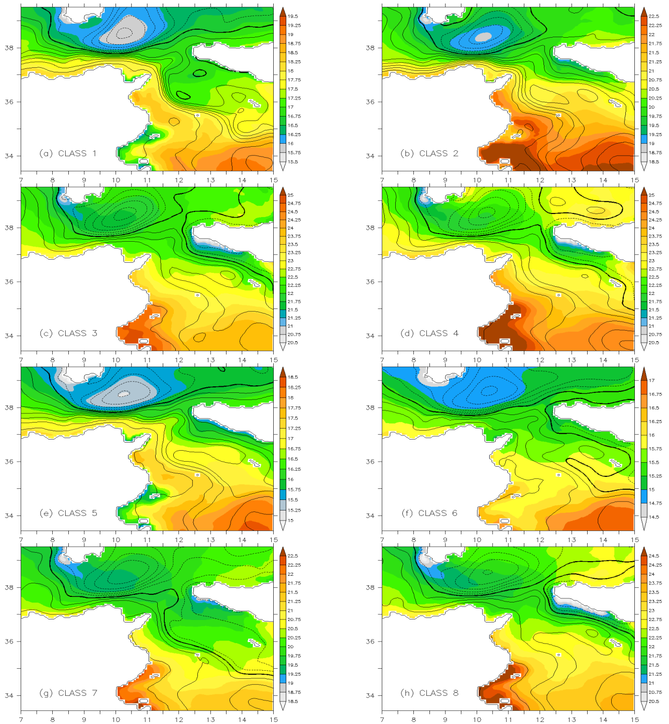
Figure 11. Sea-surface temperature ( ^{\circ}\text{C} ) for the 8 classes of Figure 5 and the associated sea-surface height anomaly represented at a contour interval of 0.02 \text{ m}\cdot\text{s}^{-1} .
