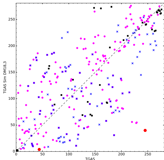
Fig. 20. Ranking of 2D subspaces according to their mutual information in the TGAS data ( x -axis) vs. the simulation ( y -axis). The black squares correspond to subspaces formed only from observables, while the blue crosses are those containing an uncertainty, and the magenta circles contain a correlation parameter. The red hexagons correspond to the subspaces shown in Fig. 21.
