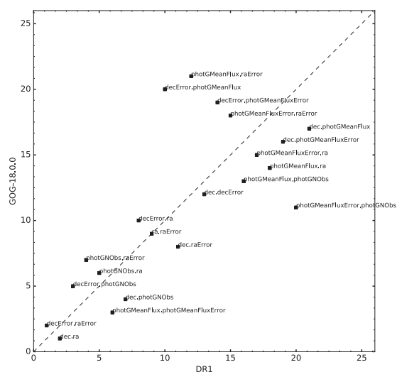
Fig. 23. Ranking of 2D subspaces according to their mutual information in the Gaia DR1 data ( x -axis) vs. the GOG simulation ( y -axis).
