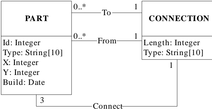
Figure 1: OO1 database schema
