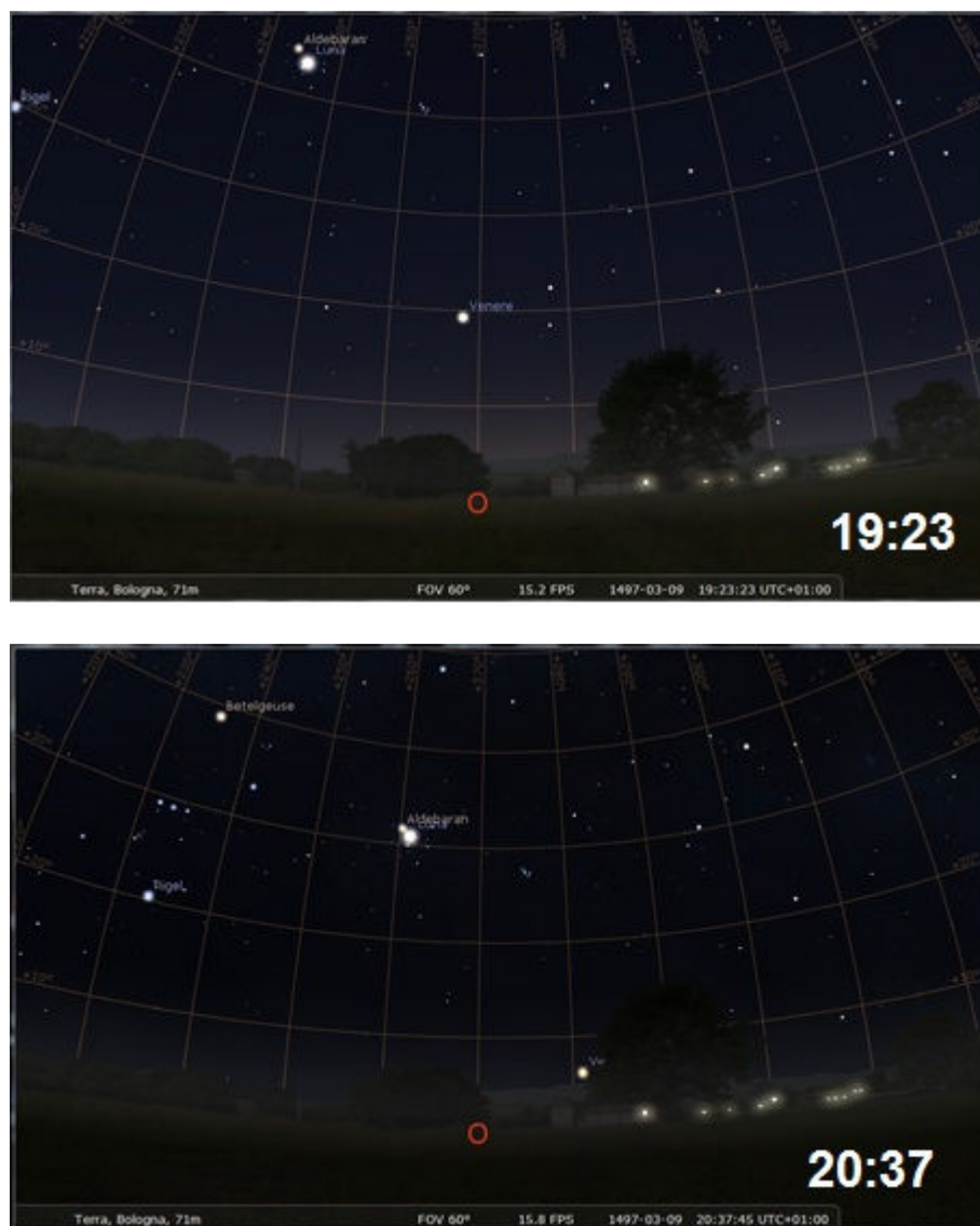
Figure 1: Observation due West (O, Ovest), from Bologna, March 9, 1497. Using Stellarium, we can see Aldebaran approaching the moon, as shown by the two snapshots.
