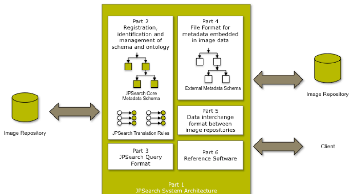
Figure 1 The global architecture of the JPSearch system.
