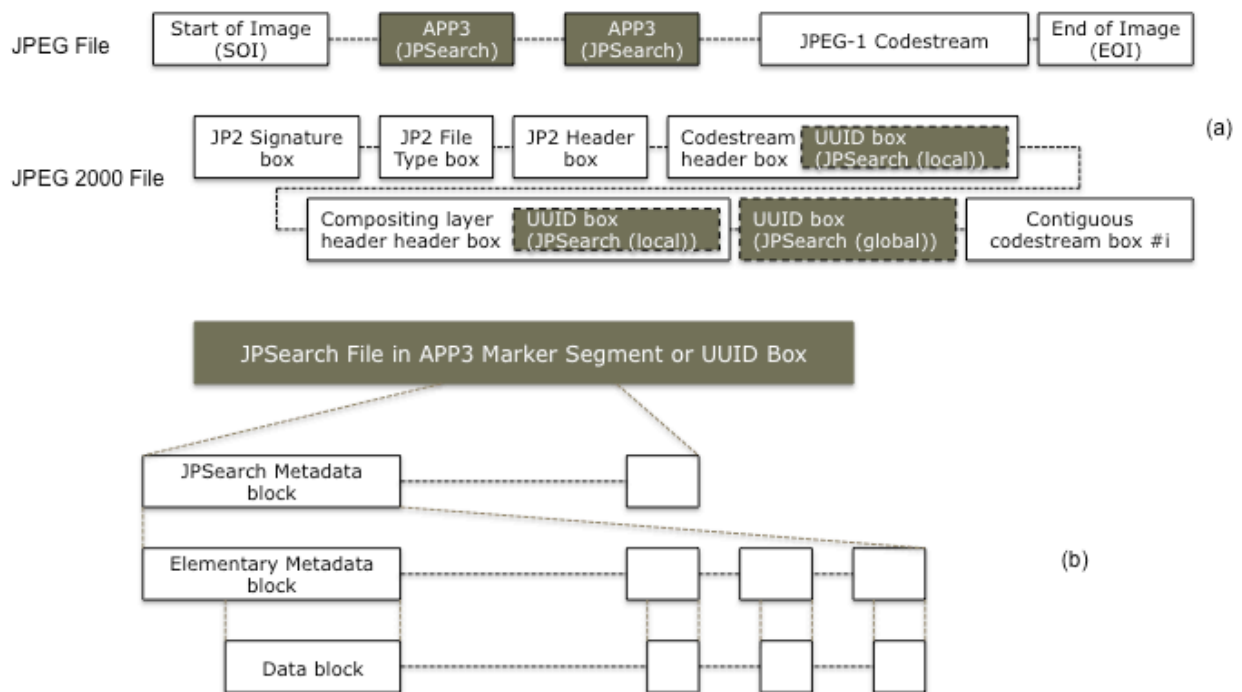
Figure 2 JPSearch files are embedded in JPEG or JPEG 2000 file formats (a), with the potential to have multiple JPSearch files carried by one image file. Each JPSearch file can contain on its turn multiple JPSearch Core Metadata Schema and Registered Schema (b). Each data block is an instance of a JPSearch Core Metadata schema (at least one) or JPSearch Registered Schema each association with a specific, potentially different author.
