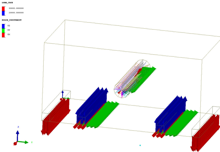
FIGURE 34. Load case for Example 18.
