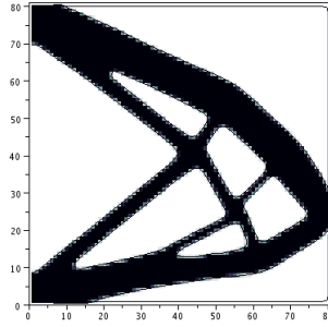
FIGURE 6. Final design for Example 1-2bis
