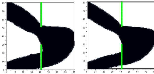
(e) Final design for the normal compliance model (f) Final design for the Coulomb model
