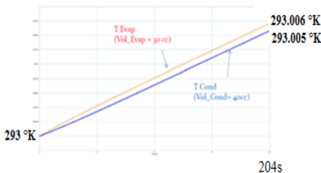
Fig 9: Temperature evolution in 1) Evaporator (orange), 2) Condenser (bleu).
