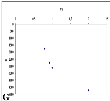
Fig.16: Methane adsorption capacity in coal seams (m 3 /ton coal) vs VR (%) after Garnier et al. (2011) in A and Hildenbrand et al. (2006) in B, and VR (%) and methane adsorption capacity (V, m 3 /ton coal) vs. depth (m) in Gironville (CD), Saulcy (EF) and Faulquemont (GH) boreholes V1 at 300 Ma, V2 at 250 Ma, V3 at 140 Ma, V4 at 0 Ma for dry coal and V4W at 0 Ma for a water content equal to 2.5 %.
