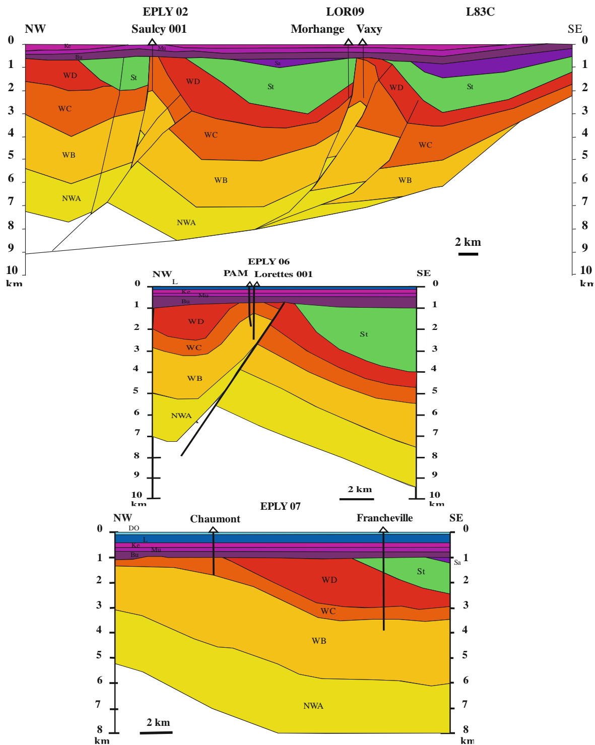
Fig. 5: Geological cross-sections based on the EPLY 02-LOR 09-L83C, EPLY 06 and EPLY 07 seismic sections
