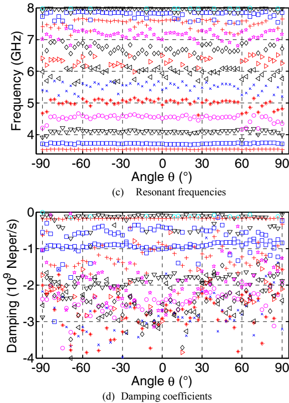
Fig. 10. Poles extracted from the measured electric far field backscattered by the helical antenna as a function of \theta .
