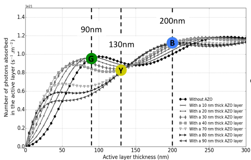
Figure 4. a) Theoretical absorption in the active layer as a function of active layer thickness (B, Y and G refers to the studied solar cells). AFM for \text{AZO}_{0.8} layers with different thickness: b) 20 nm (RMS=1.77 nm) and c) 80 nm (RMS=1.98 nm).
