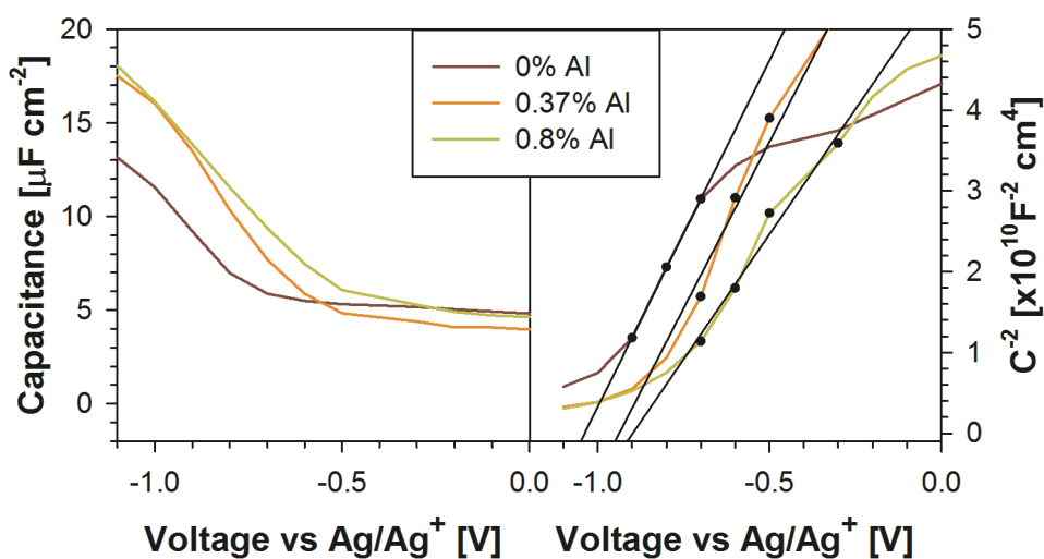
Figure 3. Mott-Schottky analysis for working electrodes in the configuration glass/ITO/AZO with different Al compositions.
