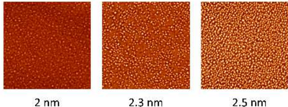
Figure 4: AFM images of a 2 \times 2 \mu\text{m}^2 area of the surface of a respectively 2, 2.3 and 2.5 nm thick \text{Si}_{0.5}\text{Ge}_{0.5} layer which were epitaxially deposited on silicon at 550 °C.
