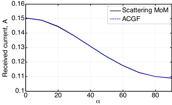
Fig. 2. Magnitude of the current received by the wire A when exciting by a plane wave as a function of the rotation of the wire B, computing both using the MoM and ACGF formalism.
