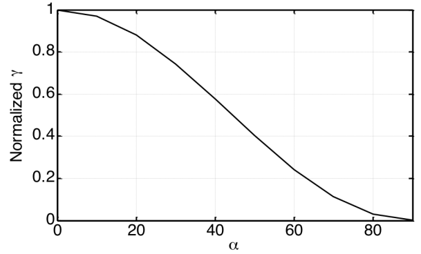
Fig. 4. Upper bound on the near-field error caused by mutual coupling as a function of the rotation of the wire B.
