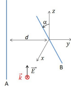
Fig. 1. The two thin wire antennas A and B with separation d . The wire B is rotated by \alpha degrees in the xz -plane.
