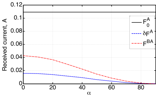
Fig. 3. Contribution of each part of the system into the current received by the wire as a function of the rotation of the wire B.
