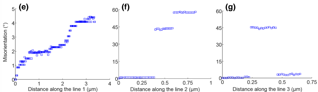
Figure 2: ACOM phase and orientation maps in the aged condition showing the microstructure of martensite, the spatial distribution of austenite. (a) and (b) phase and orientation maps of a first area. (c) and (d) phase and orientation maps of a second zone (quality index is superimposed to these two maps to illustrate the microstructure within the martensite laths). (e), (f) and (g) misorientation profiles for the linescans shown in figure (d), respectively within martensite, across a martensite grain boundary containing a martensite island, and across an austenite island embedded in martensite.
