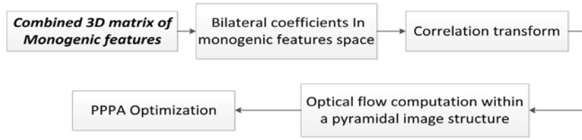
Figure 2. Flowchart of the proposed motion estimation method.
